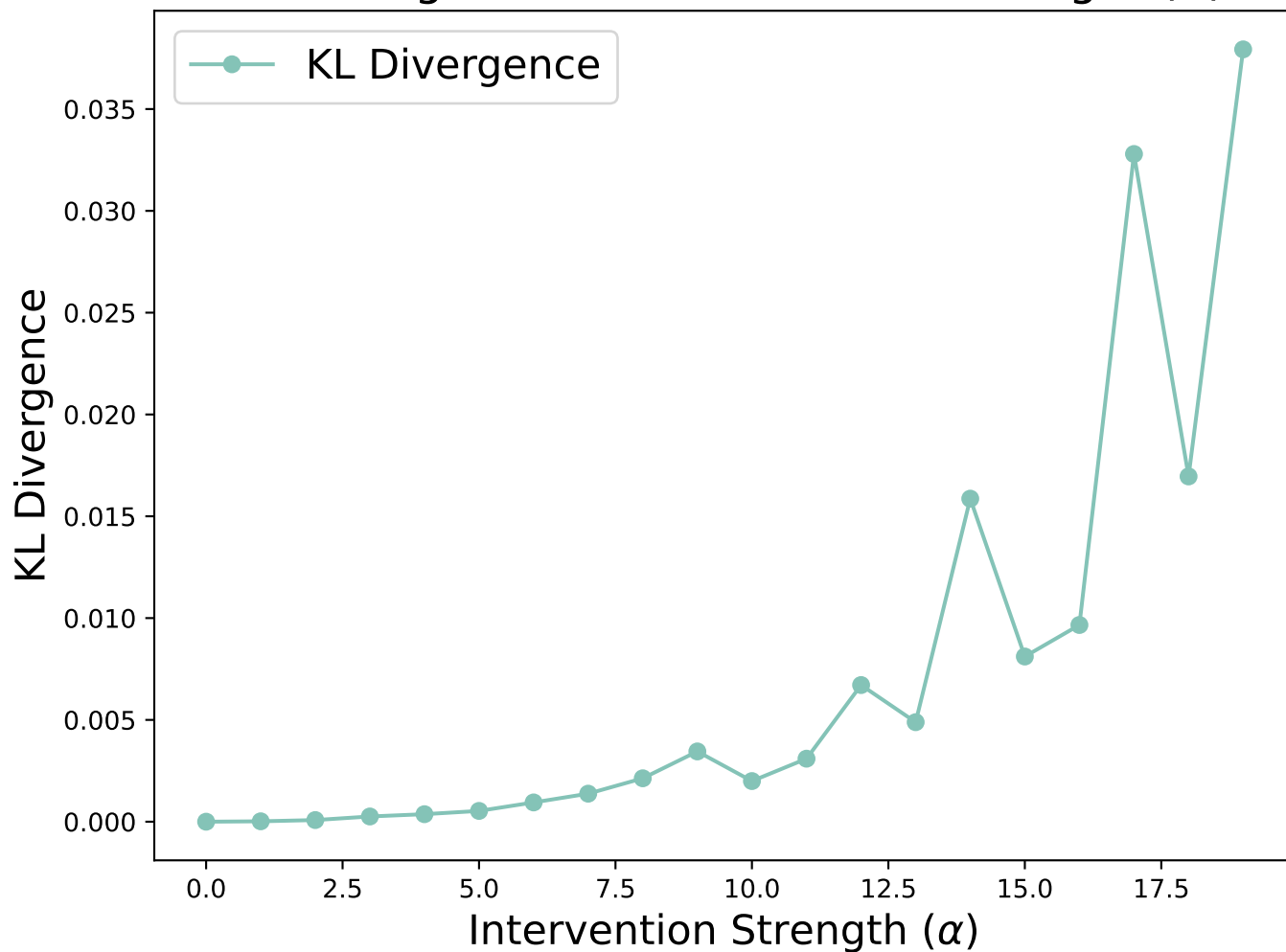
KL Divergence vs. Intervention Strength ( \alpha )
