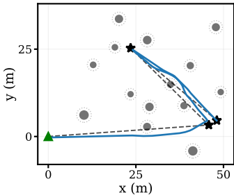
A1 opus-5 #1: PASS min clearance 1.65 m
