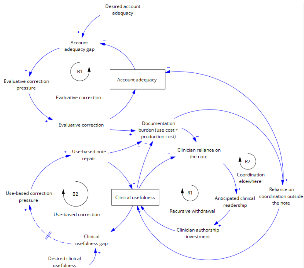
Figure 4: Reinforcing loop 2.
