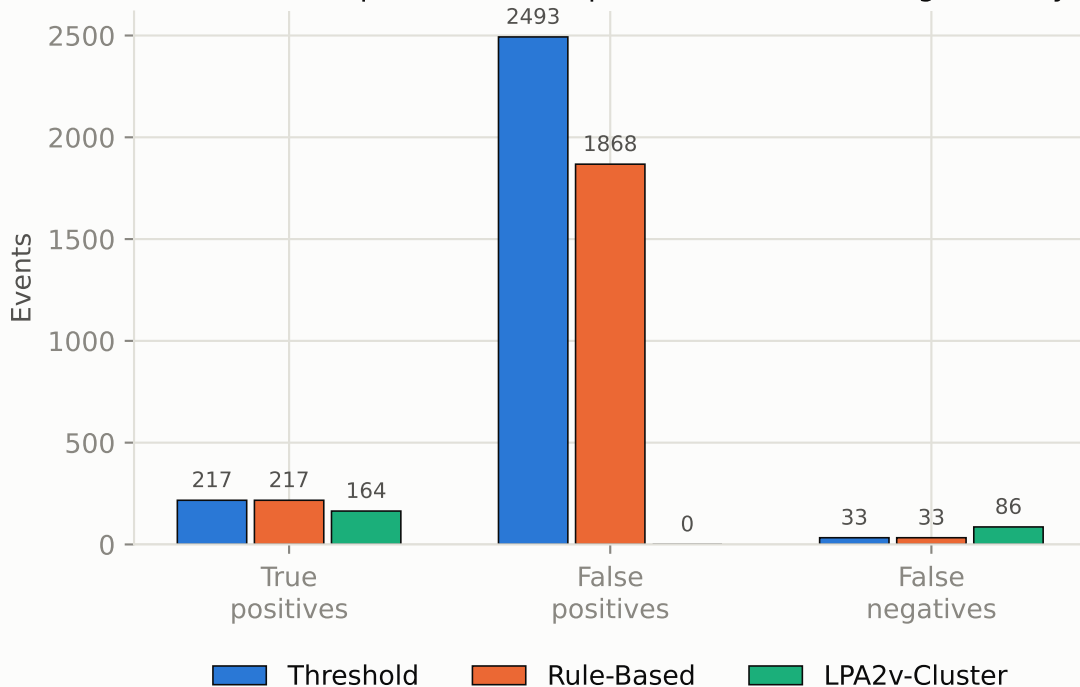
Volume of true positives, false positives, and false negatives by mechanism
