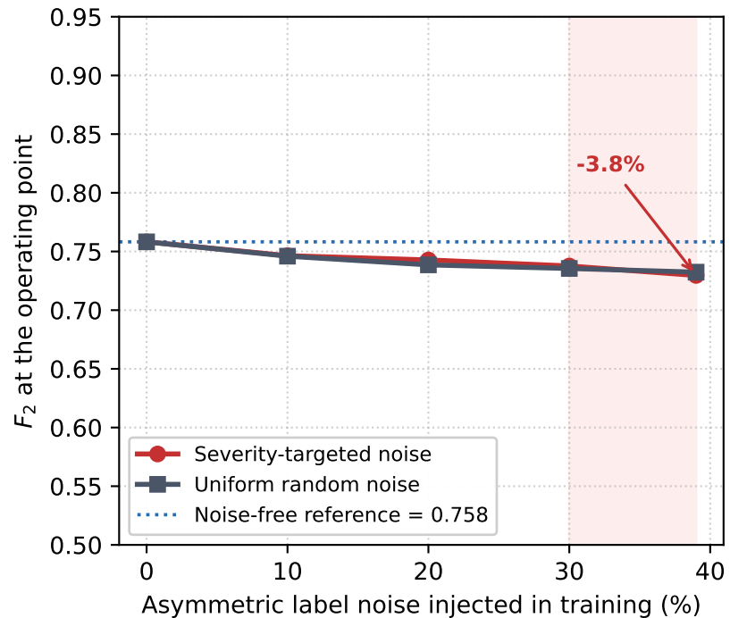
Robustness of the supervised model to label noise (shaded band = 39% inconsistency rate reported by Klimes-Dougan et al., 2022)
