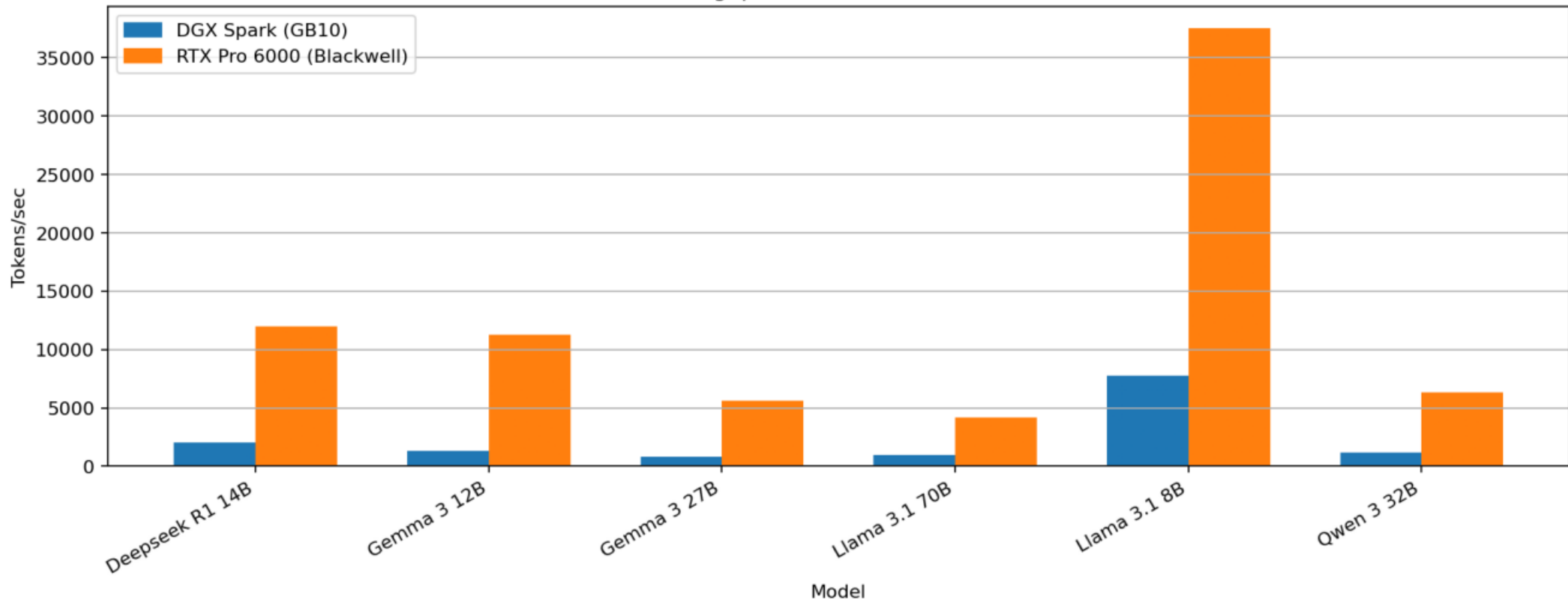
Prefill Throughput (Tokens/sec) — Batch Size 8
