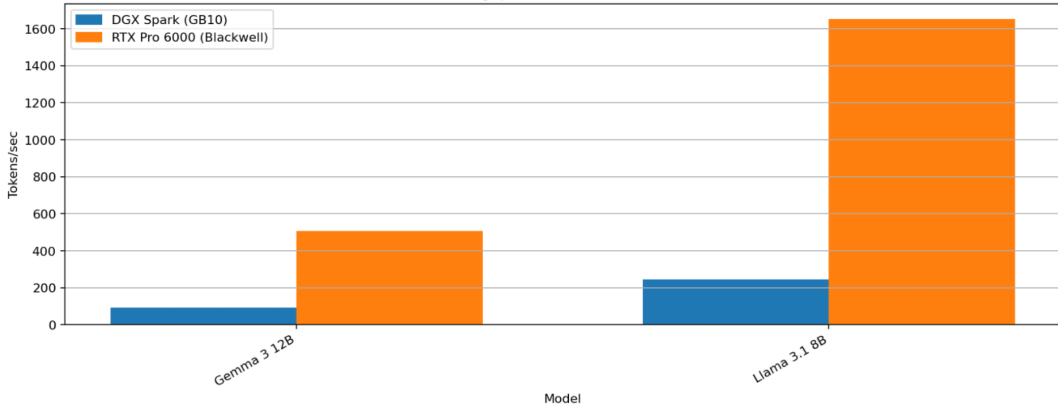
Decode Throughput (Tokens/sec) — Batch Size 16
