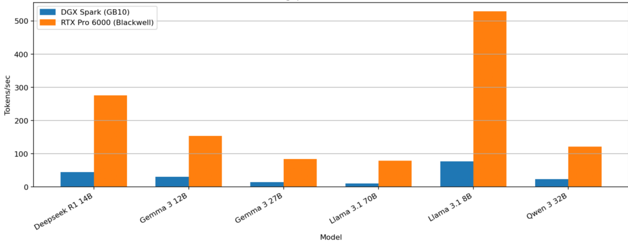
Decode Throughput (Tokens/sec) — Batch Size 4
