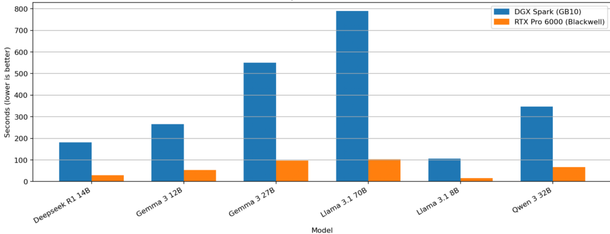
Estimated E2E Latency (s) — 2k in / 2k out — Batch Size 4
