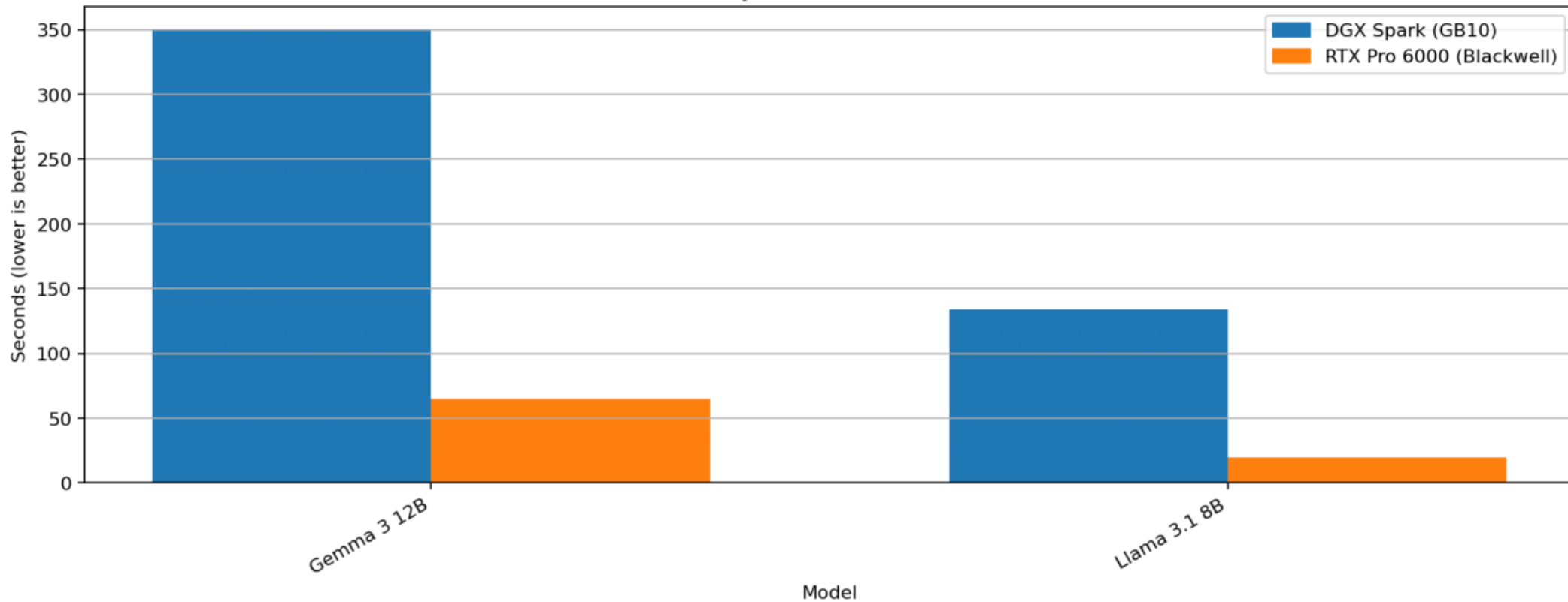
Estimated E2E Latency (s) — 2k in / 2k out — Batch Size 16
