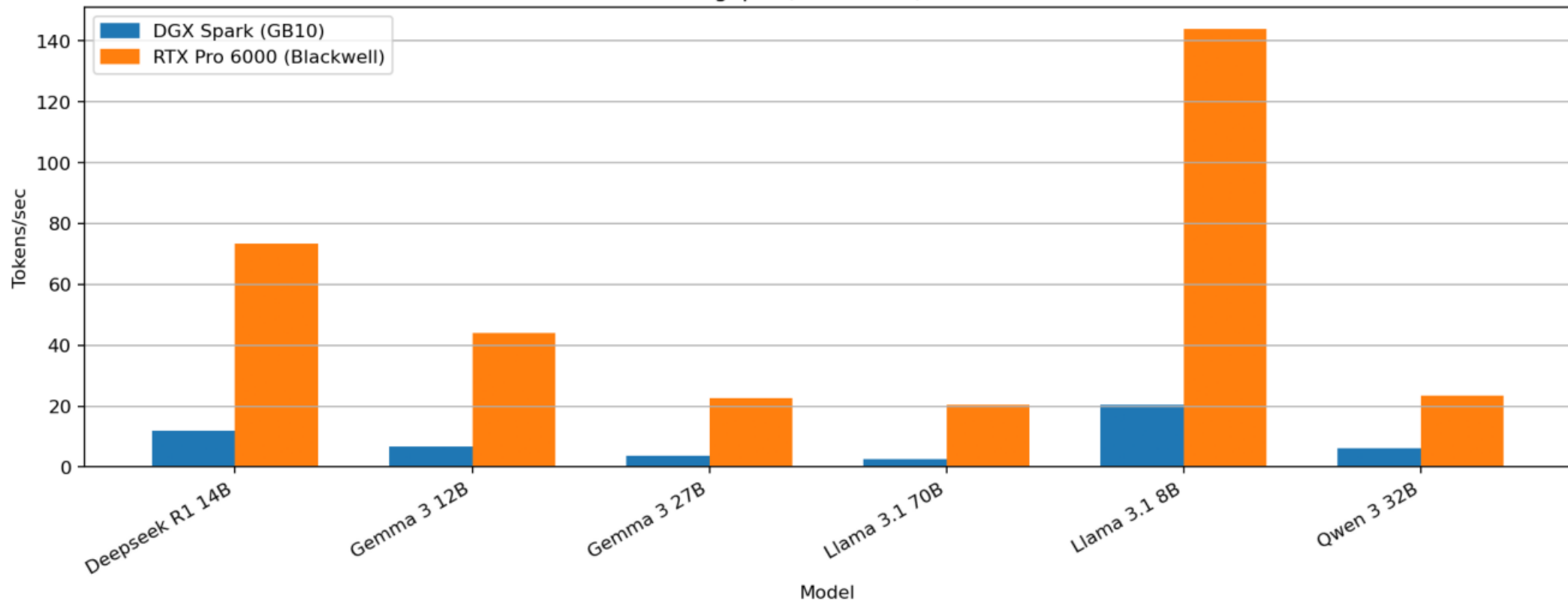
Decode Throughput (Tokens/sec) — Batch Size 1
