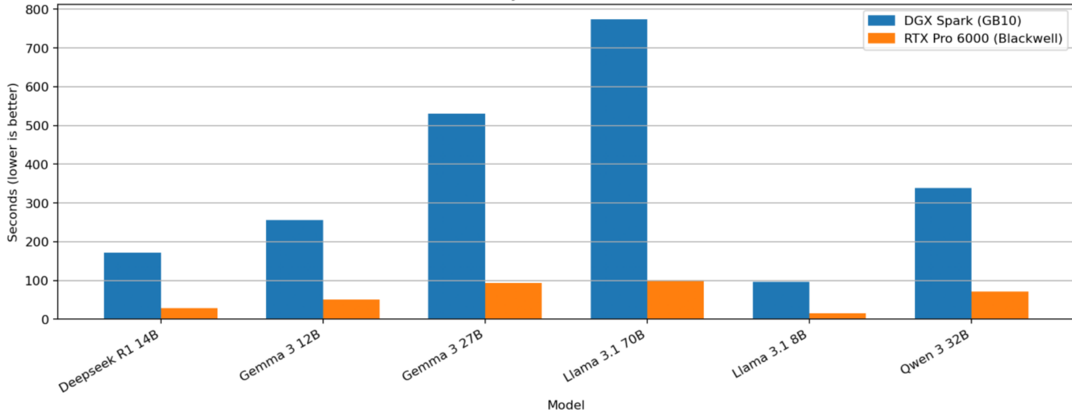
Estimated E2E Latency (s) — 2k in / 2k out — Batch Size 2
