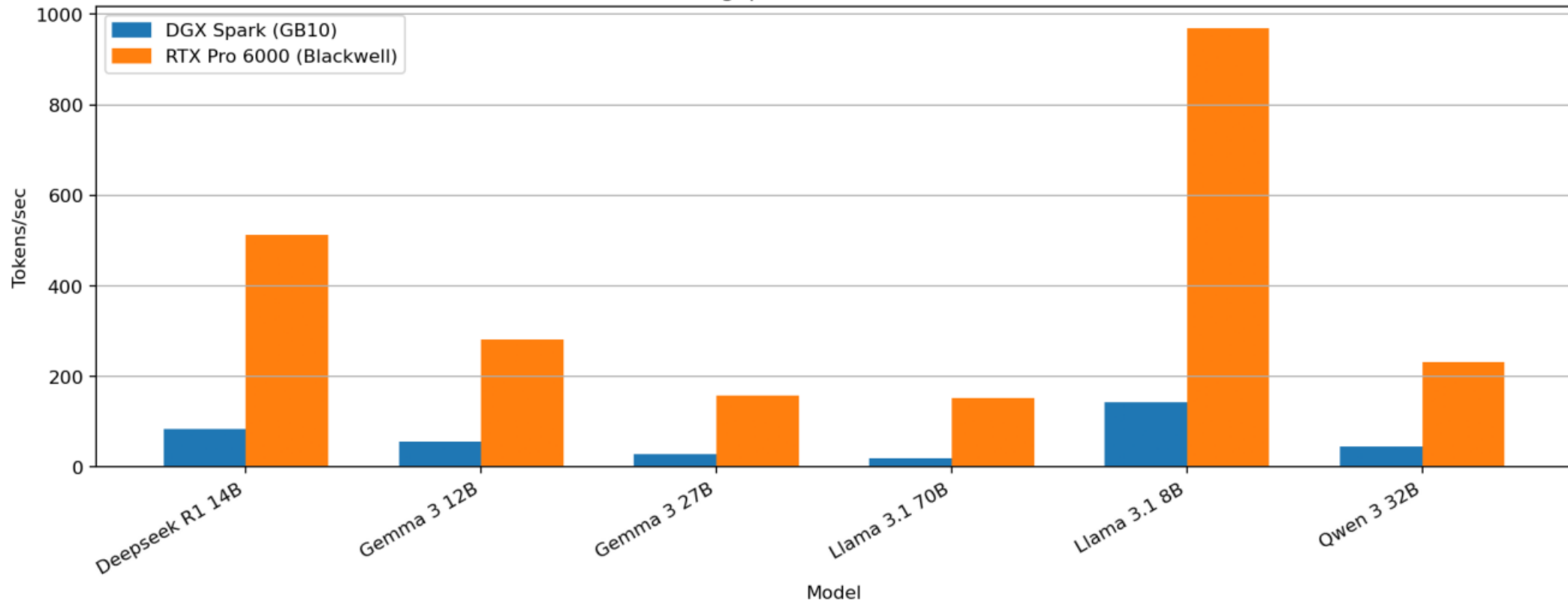
Decode Throughput (Tokens/sec) — Batch Size 8
