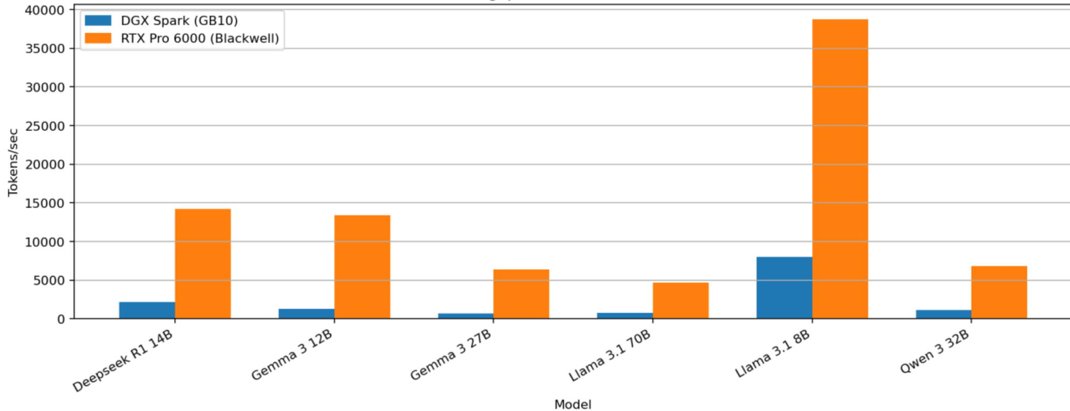
Prefill Throughput (Tokens/sec) — Batch Size 1
