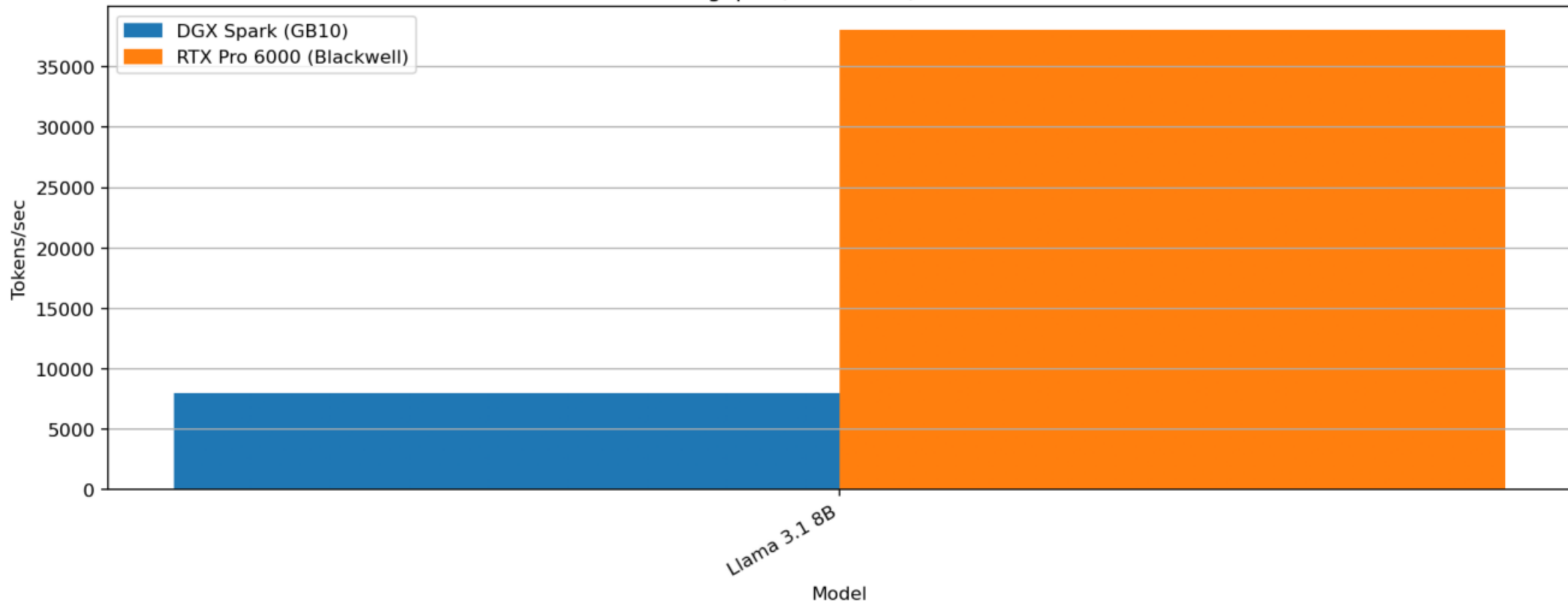
Prefill Throughput (Tokens/sec) — Batch Size 32
