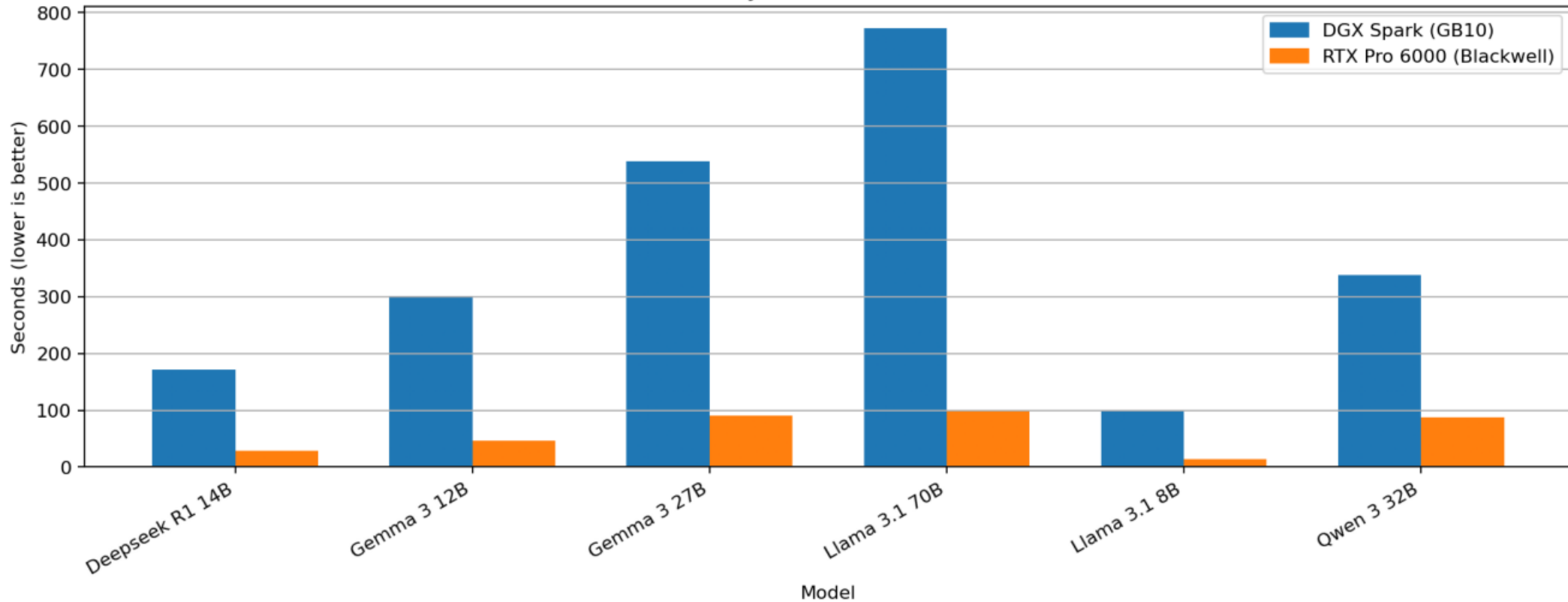
Estimated E2E Latency (s) — 2k in / 2k out — Batch Size 1
