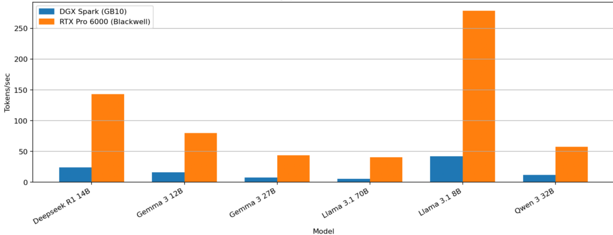
Decode Throughput (Tokens/sec) — Batch Size 2
