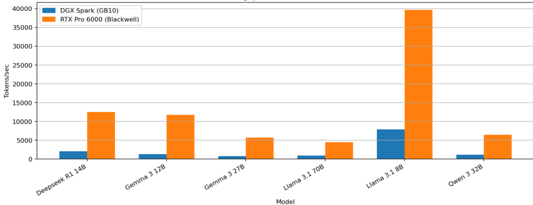
Prefill Throughput (Tokens/sec) — Batch Size 4
