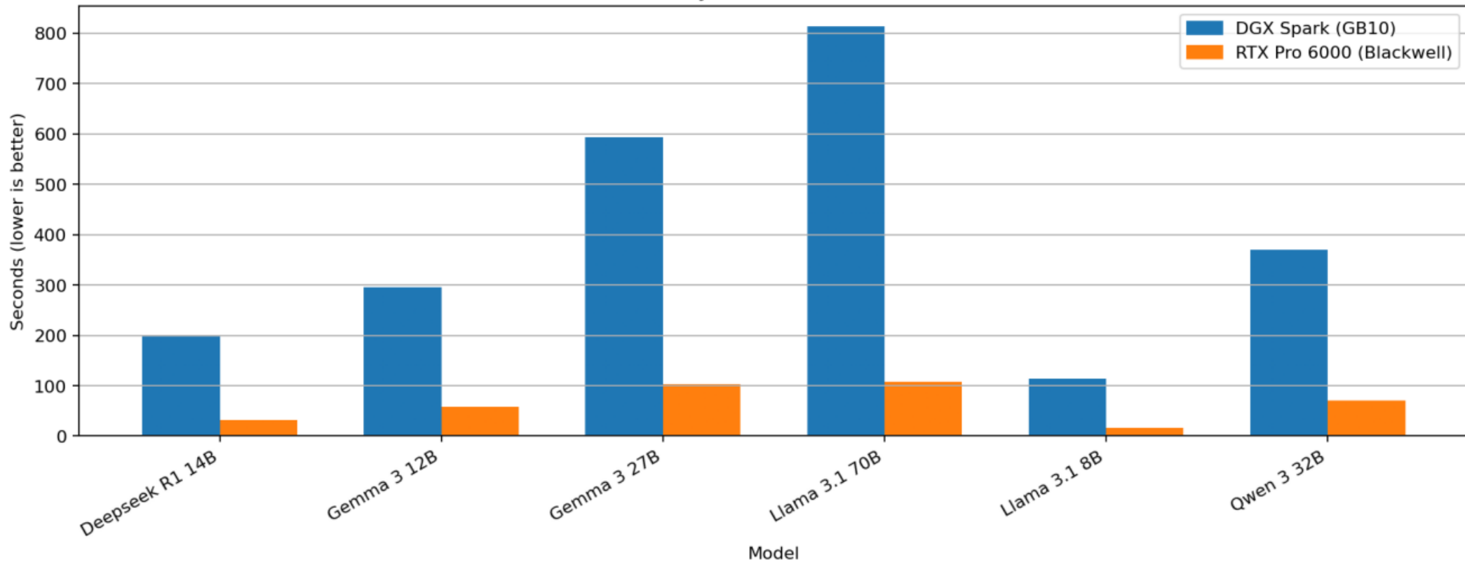
Estimated E2E Latency (s) — 2k in / 2k out — Batch Size 8
