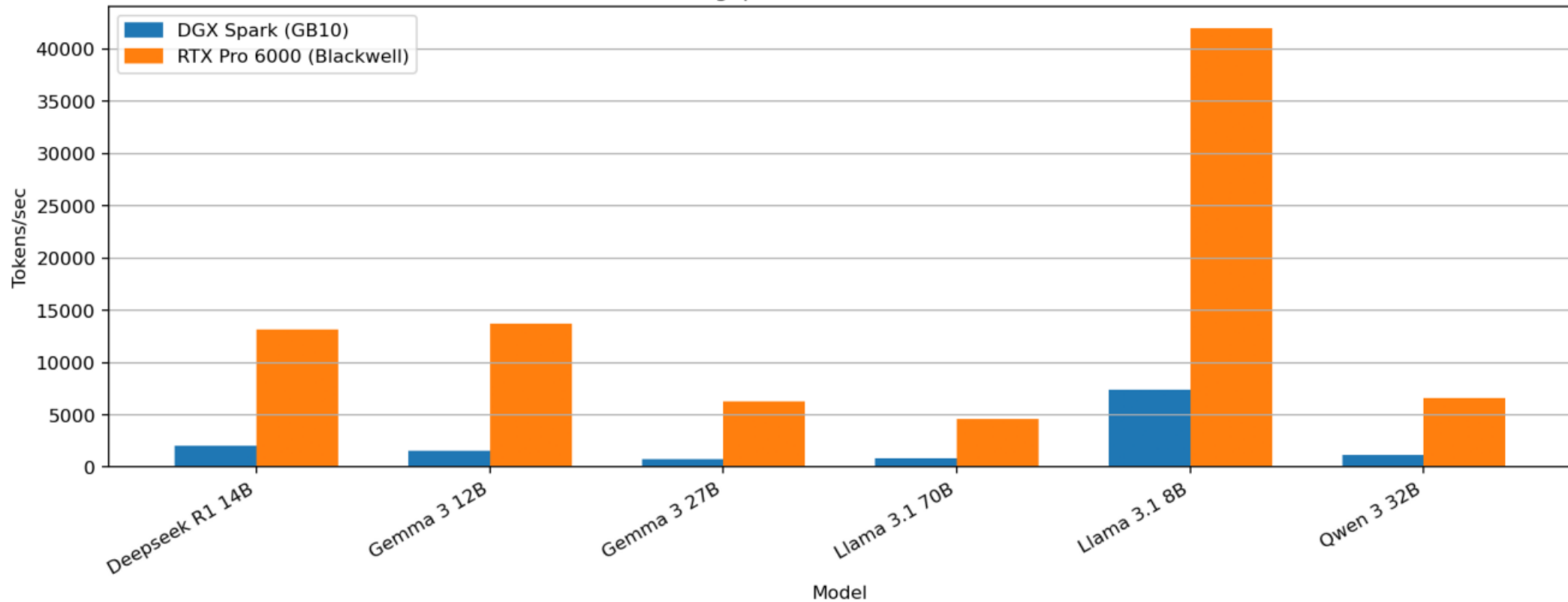
Prefill Throughput (Tokens/sec) — Batch Size 2
