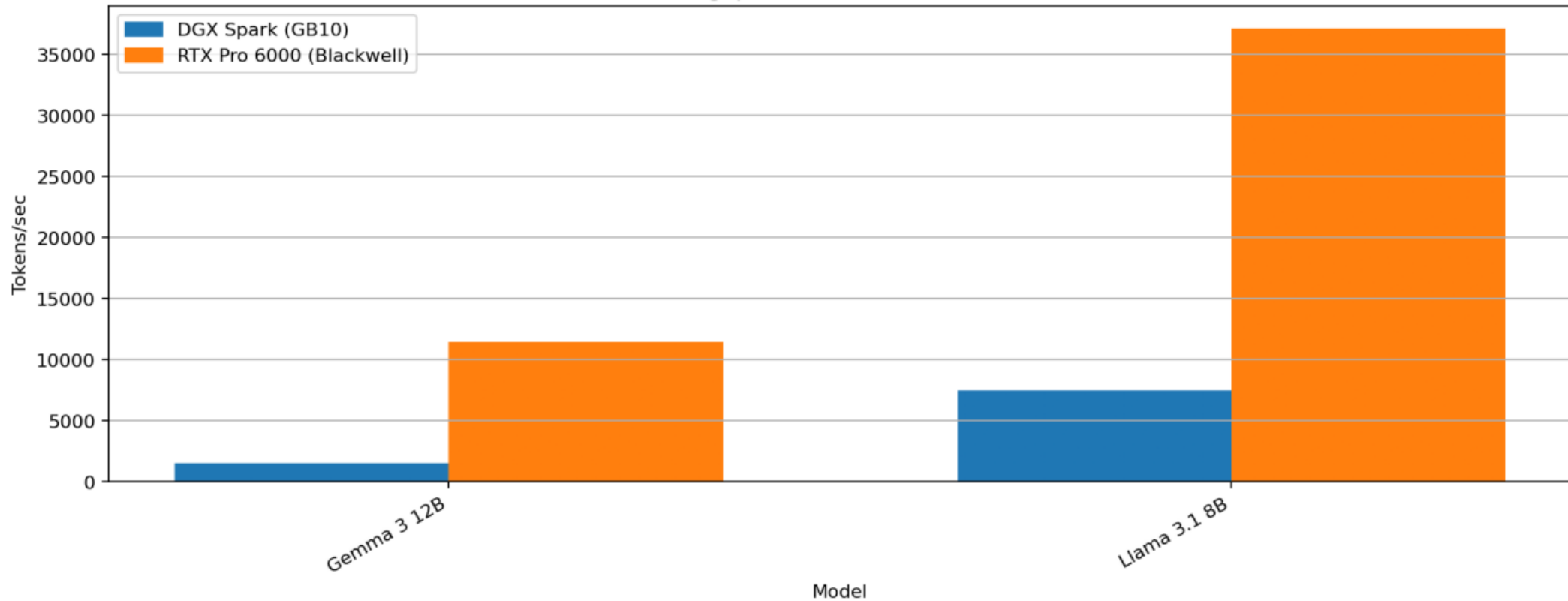
Prefill Throughput (Tokens/sec) — Batch Size 16
