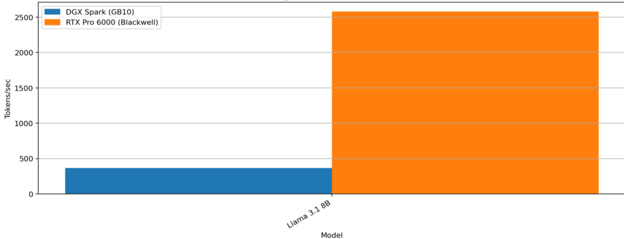
Decode Throughput (Tokens/sec) — Batch Size 32
