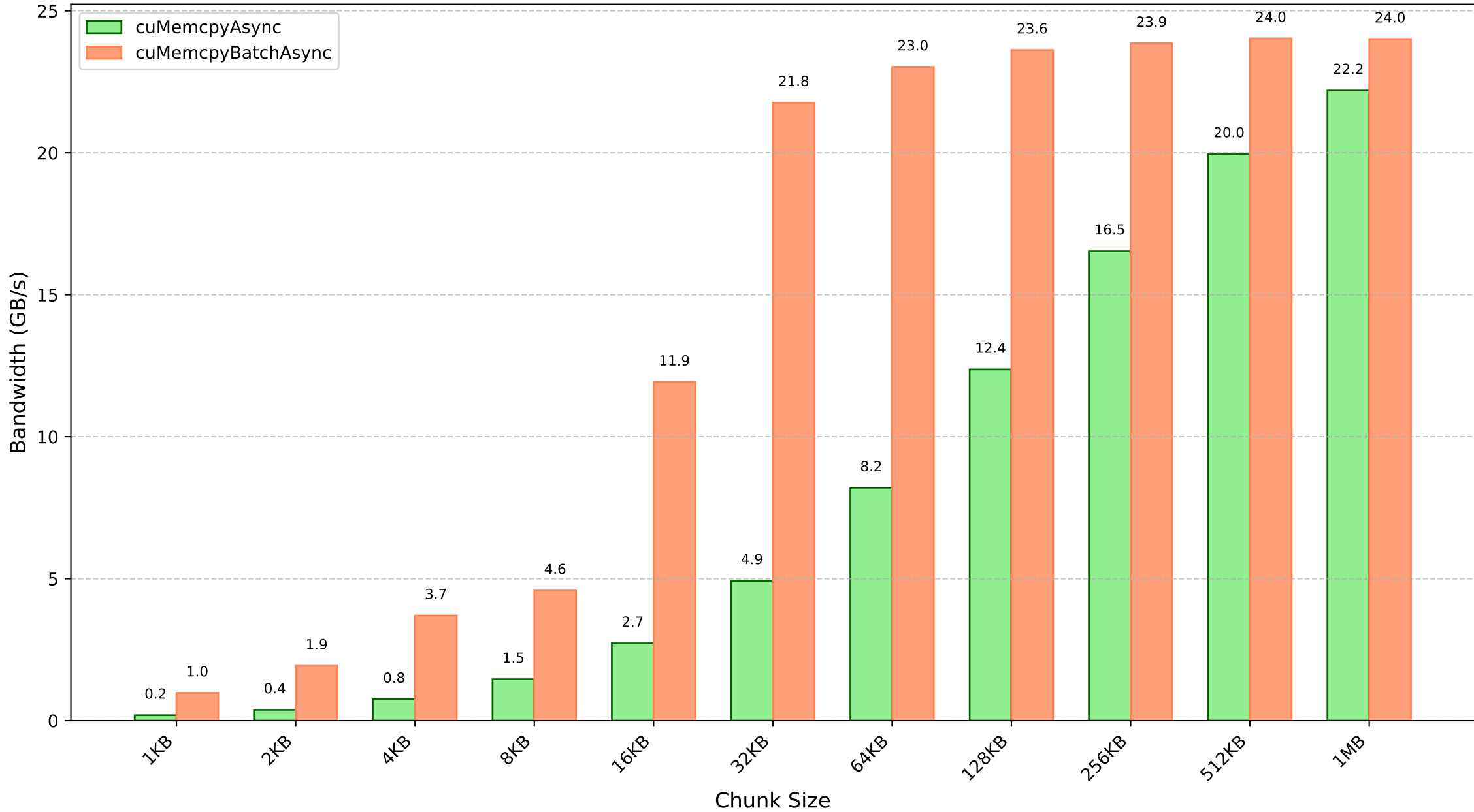
D2H Comparison of Bandwidth vs Chunk Size (32MB Data)
