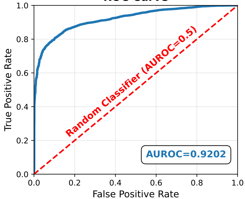
ROC Curve
