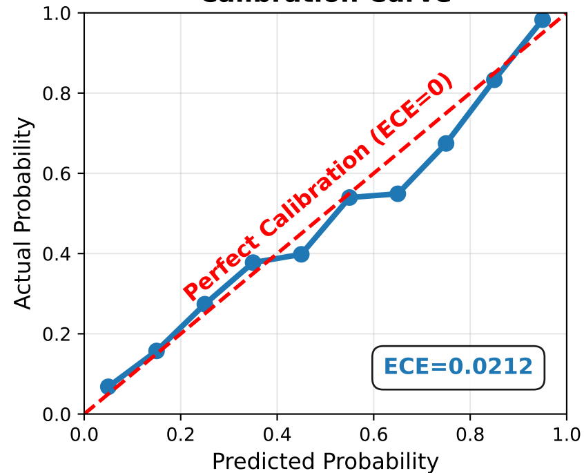
Calibration Curve
