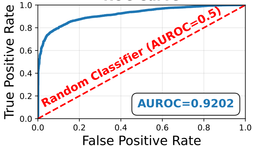
ROC Curve
