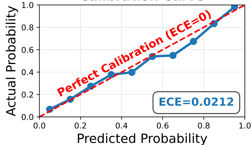
Calibration Curve
