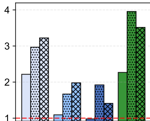
(c) OPT-30B / OPT-350M (10 req/s, H200)
