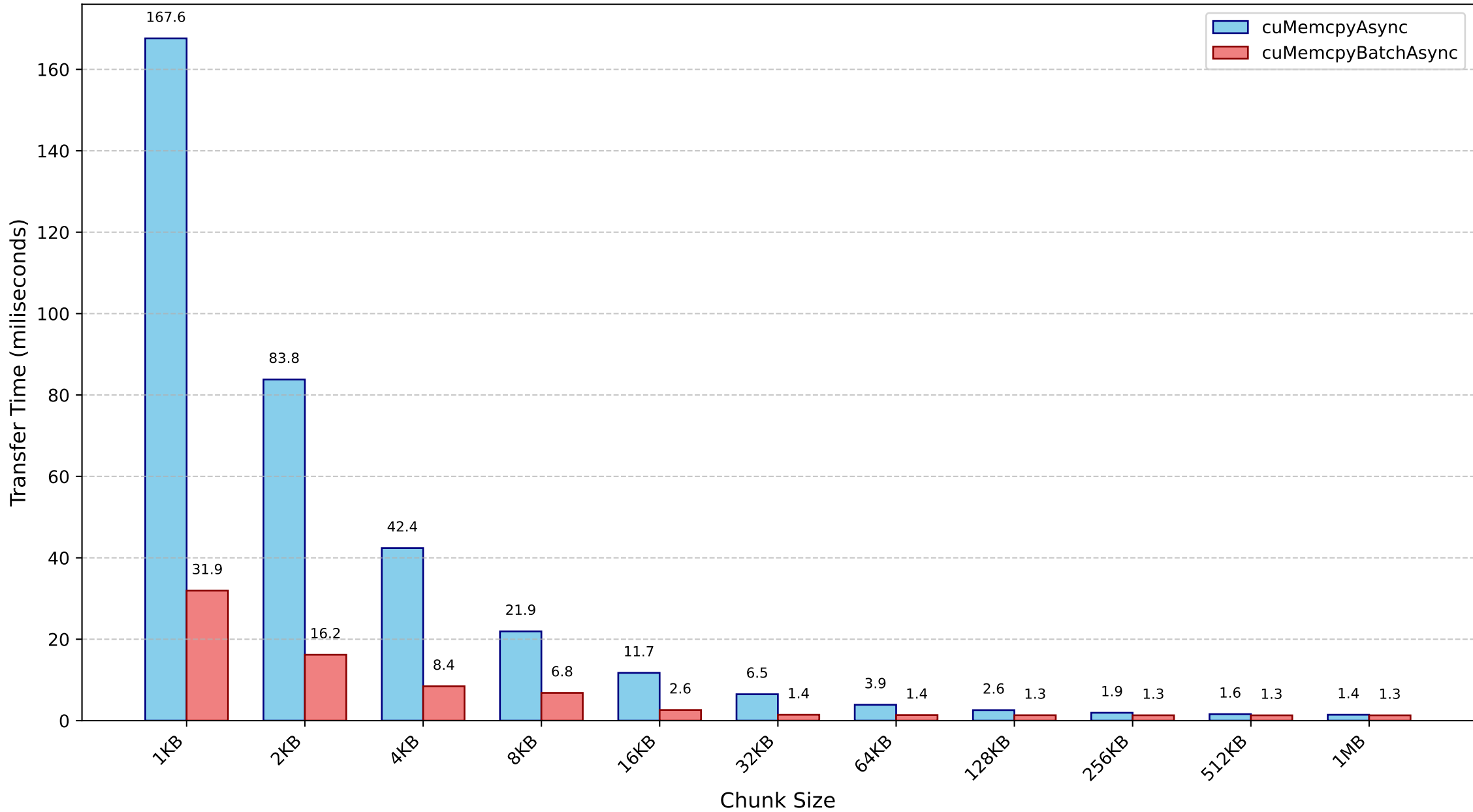
D2H Comparison of Transfer Time vs Chunk Size (32MB Data)
