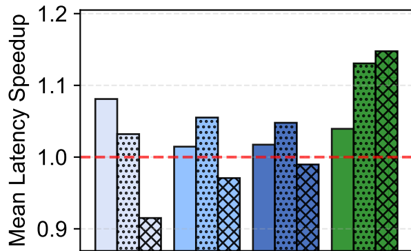
(a) OPT-6.7B / OPT-125M (10 req/s, A6000)
