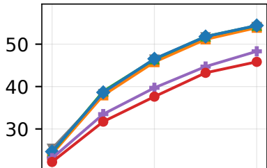
GPT-OSS-120B
