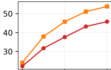
GPT-OSS-120B
