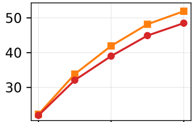
GPT-OSS-120B
