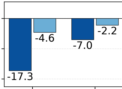
GPT-OSS-120B
