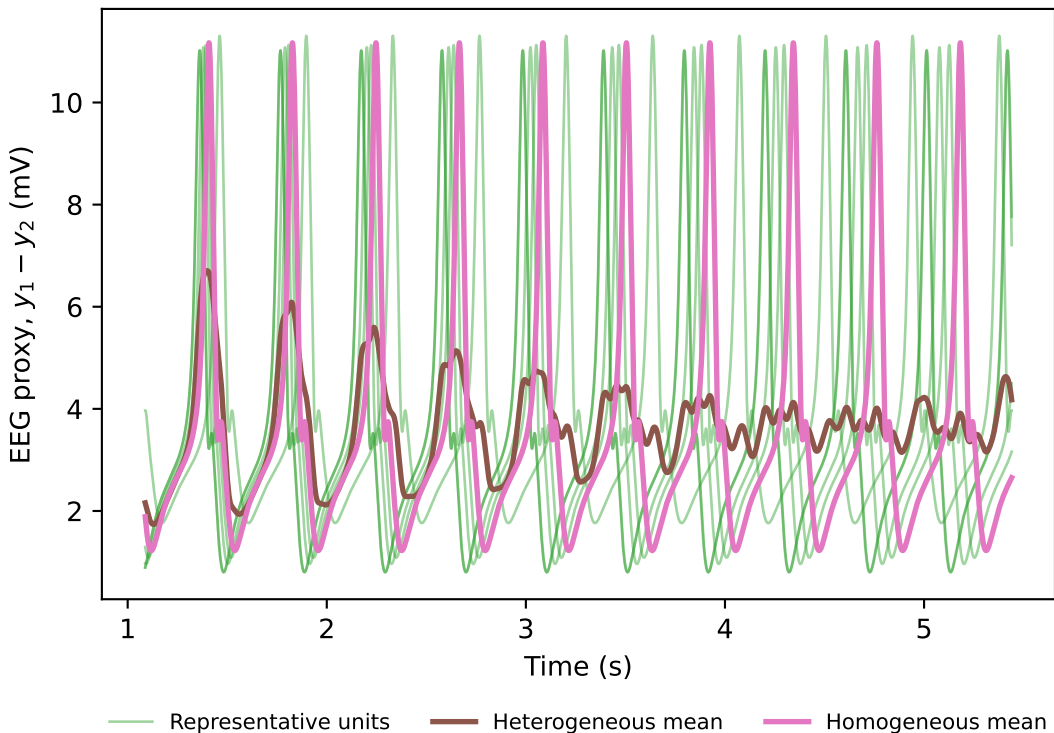
Jansen-Rit: v_0 heterogeneity ( h = 0.75 )
