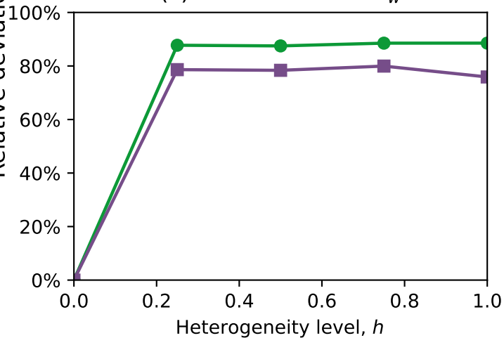
(c) FHN timescale: \tau_w
