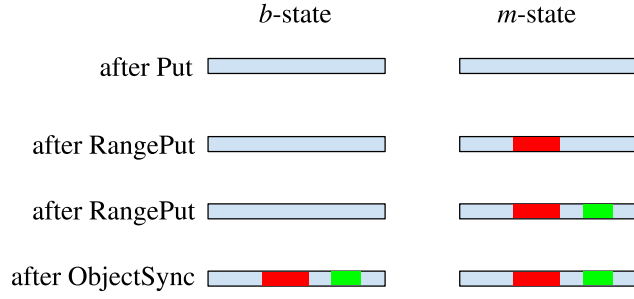
Figure 1: Object b - and m -states across three operations. Colored bars represent modified portions of the object state.
