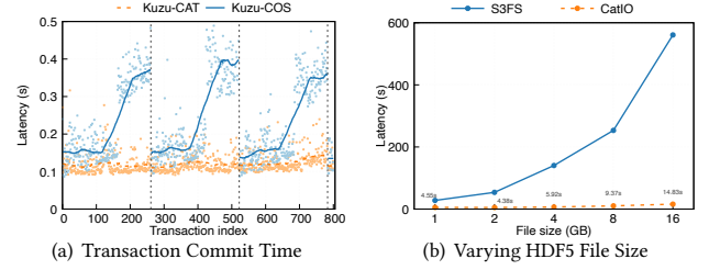
Figure 9: The performance of Cat's use cases.
