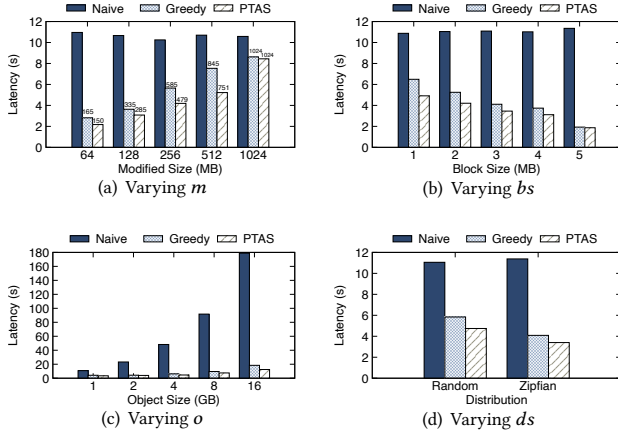
Figure 8: The performance of Publish
