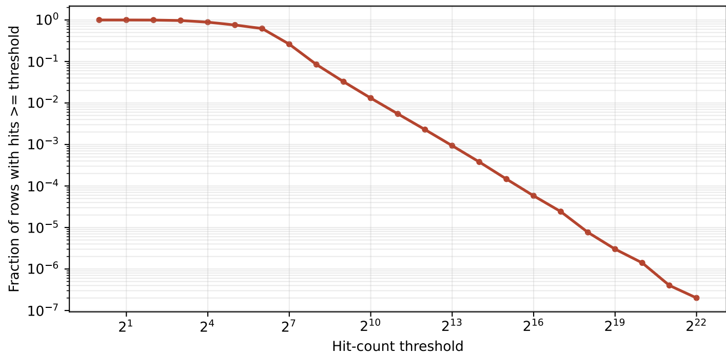
Hit-count CCDF
