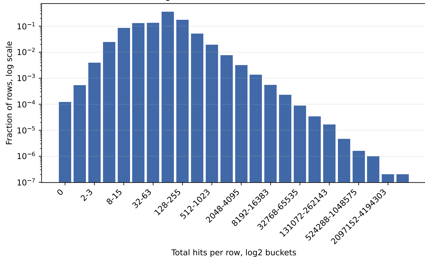
Engram row hit-count distribution
