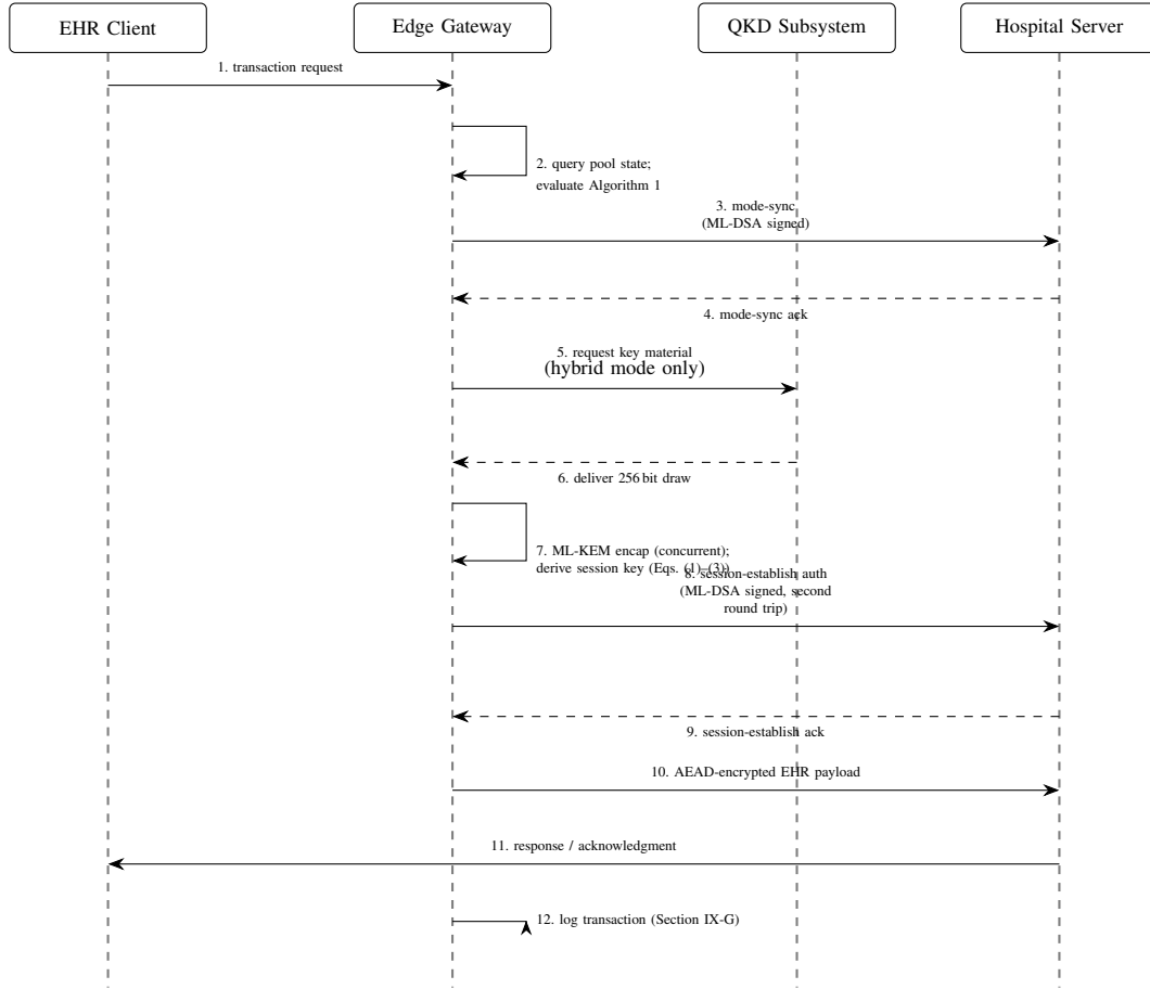
Fig. 2. Adaptive (B5) key-establishment message sequence for the normal flow (QKD available), traced directly from B5Adaptive.establish_session_key() ( src/baselines/baselines.py ) rather than from an idealized protocol description. Steps 5–6 (QKD draw) and step 7 (ML-KEM encapsulation) occur concurrently, not sequentially, as drawn here only for message-ordering clarity. Two separate authenticated round trips occur, not one: mode-sync (steps 3–4), before key material is drawn — confirming which path the receiver should expect — and a second, independent session-establish authentication (steps 8–9) after the session key is derived, mutually confirming the established session itself; this is why B5’s measured overhead (Section XI) is exactly two ML-DSA signature round trips (6618 bytes) larger than B4’s single round trip, not one. In the degraded and unavailable flows (also described in Section V’s Data Flow), step 2’s decision instead routes through the bounded-wait or immediate-PQC-only branches of Algorithm 1, and steps 5–6 are skipped entirely when the controller resolves to PQC-only — steps 3–4 and 8–9 still occur in that case, since both authenticated round trips are unconditional in the implementation.
