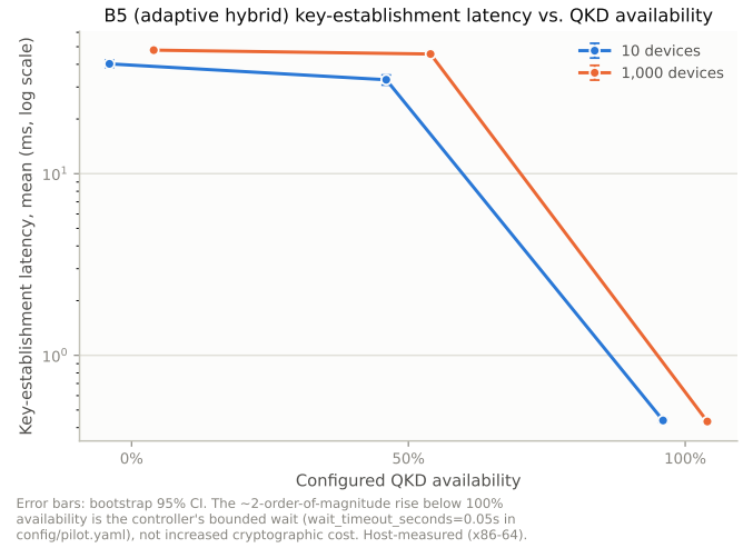
Fig. 2. B5 key-establishment latency (mean, bootstrap 95% CI, log scale) vs. QKD availability, by device count.
