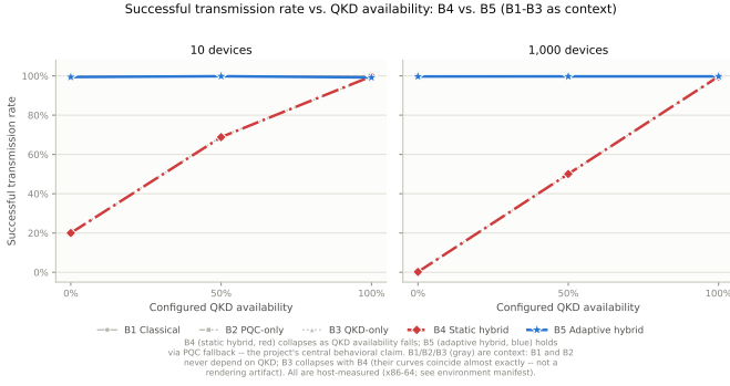
Fig. 1. Successful transmission rate vs. QKD availability. B4 (red) and B5 (blue) are emphasized as the paper’s central comparison; B1–B3 (gray) are context and, for B1/B2/B5-at-full-availability and for B3/B4, are numerically near-coincident (see caption in figure).
