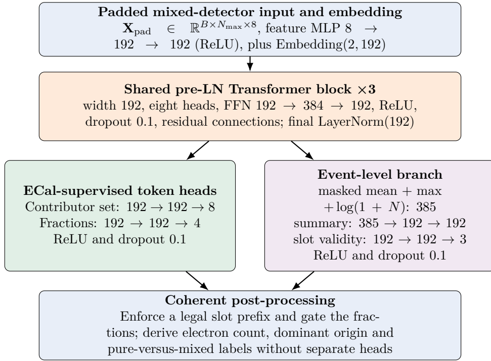
Figure 1: Architecture of the selected MLPF-inspired contributor-set slot model. The eight contributor-set classes encode all subsets of three electron slots; the four fraction components represent background and the three slots.
