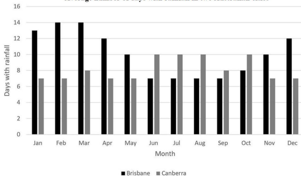
Average number of days with rainfall in two Australian cities
