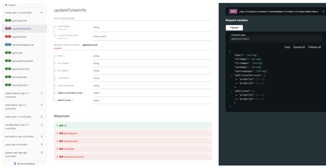
Fig. 7. API contract validation portal (Redoc/OpenAPI).
