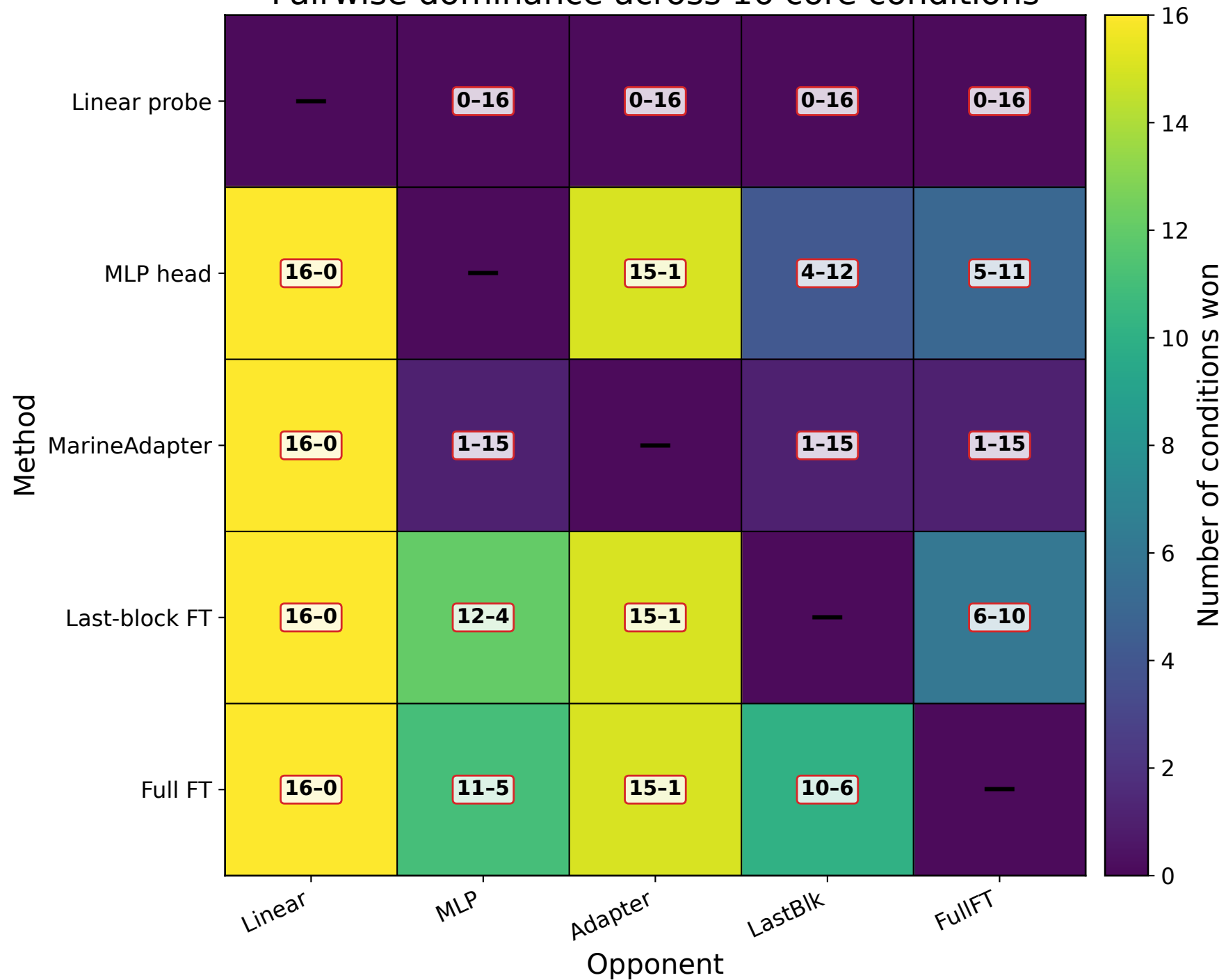
Pairwise dominance across 16 core conditions
