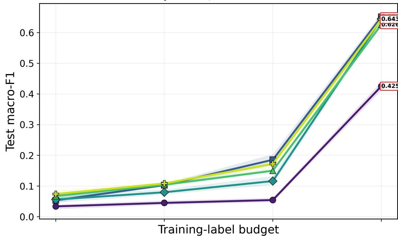
AQUA20 / ResNet-18
