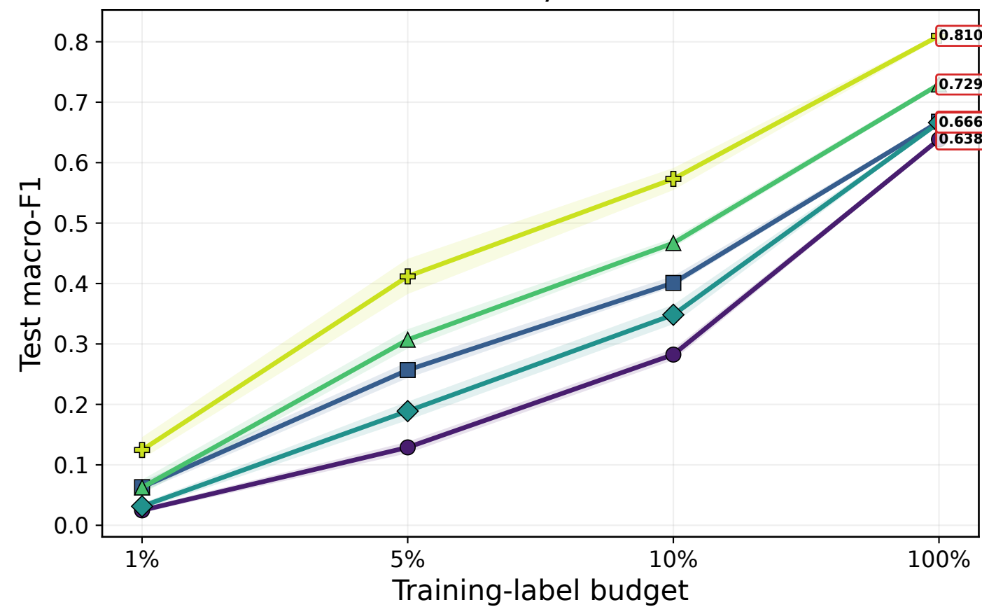
FathomNet / DINOv2-S
