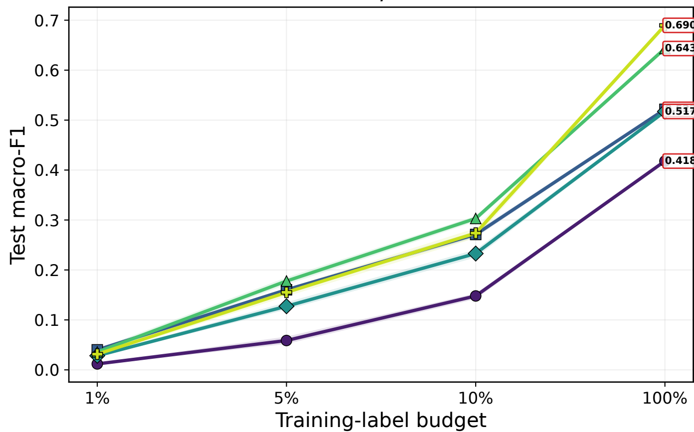
FathomNet / ResNet-18
