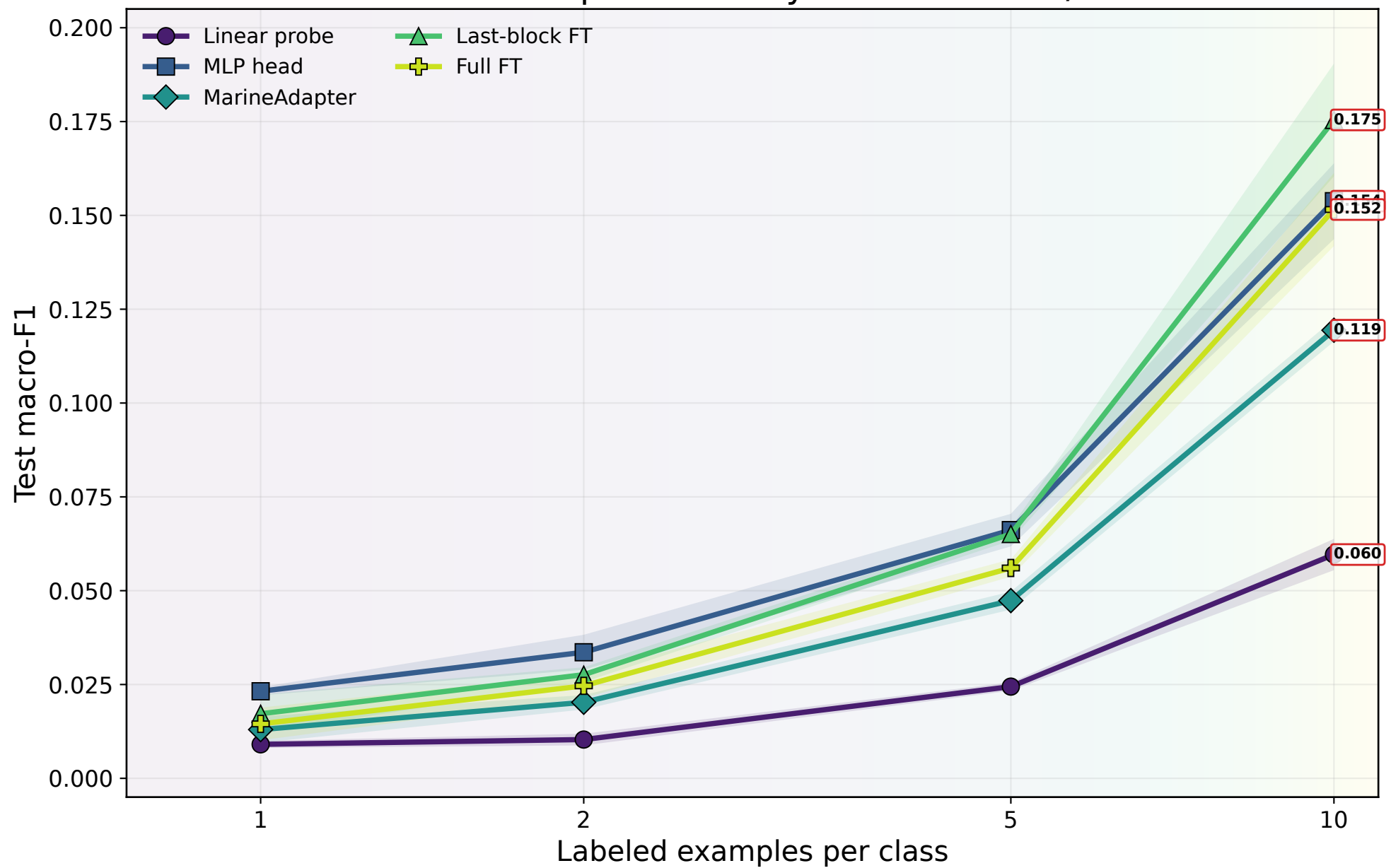
Class-balanced sample efficiency on FathomNet / ResNet-18
