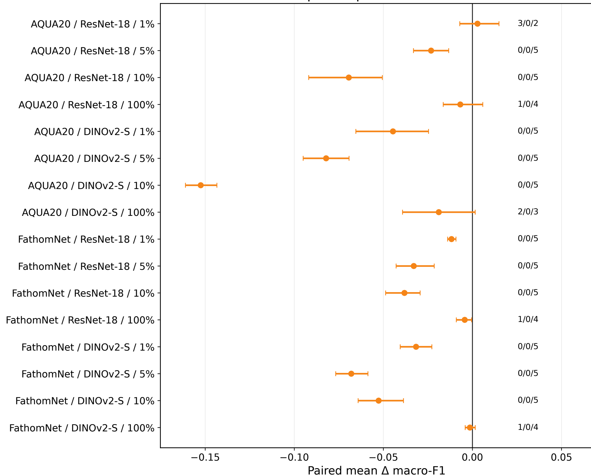
MarineAdapter vs parameter-matched MLP w/T/L
