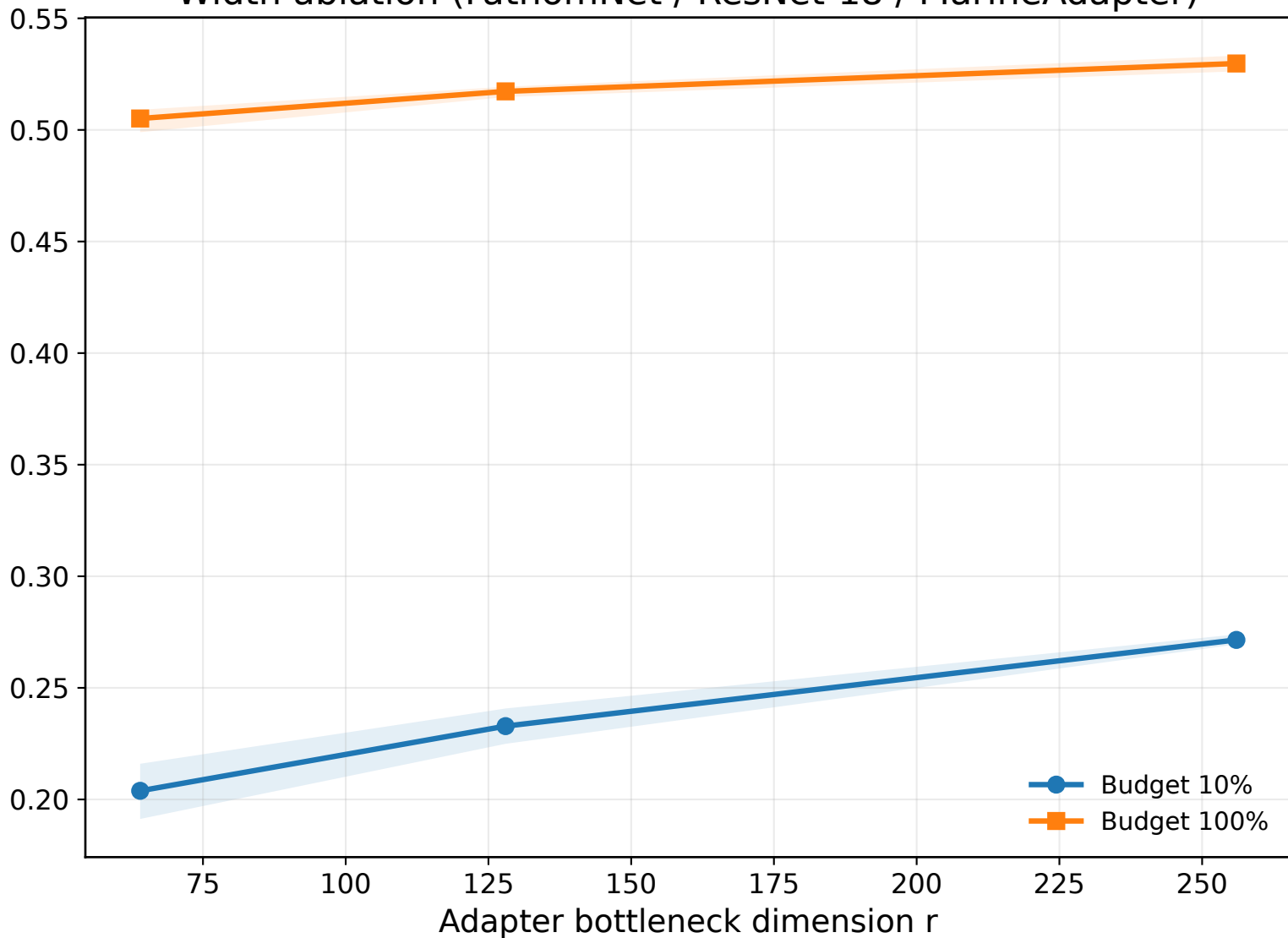
Width ablation (FathomNet / ResNet-18 / MarineAdapter)
