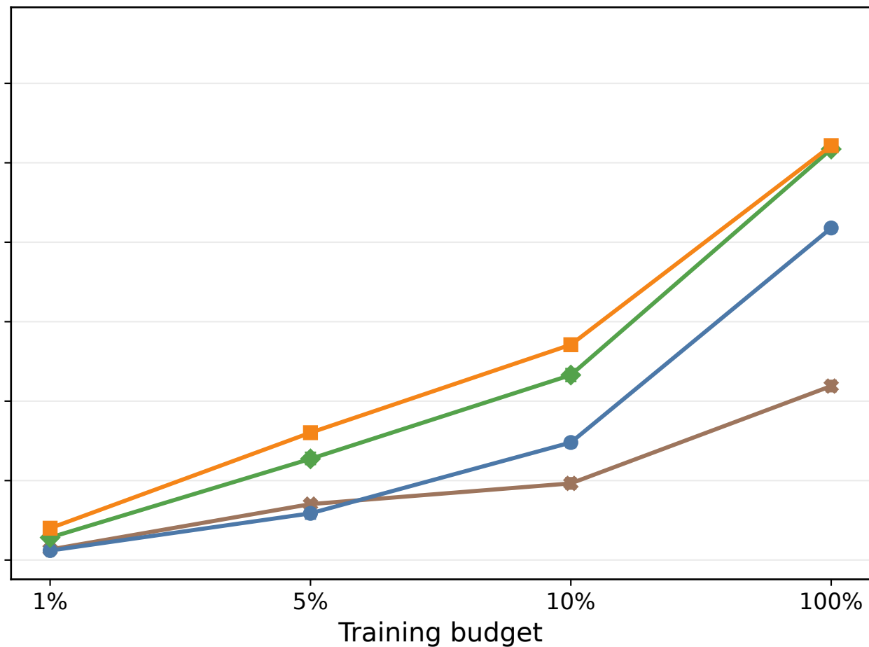
FathomNet
