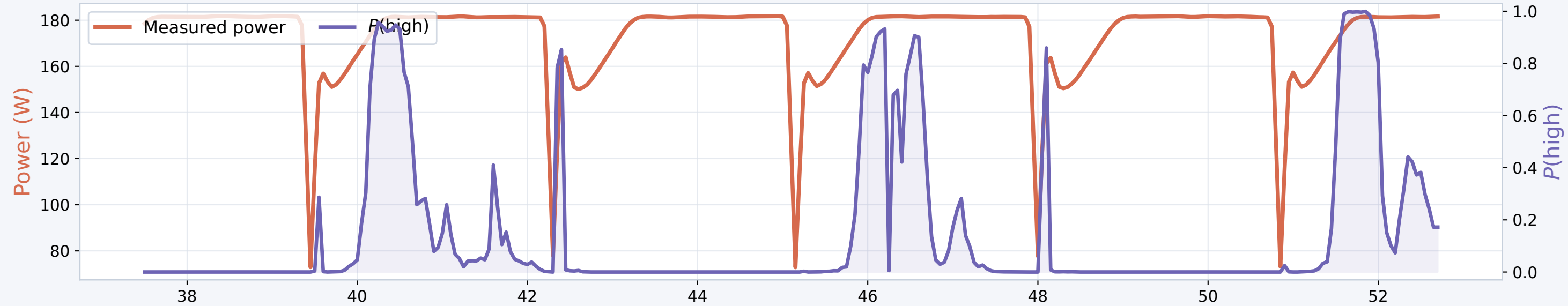
Melt-pool response in the same interval
