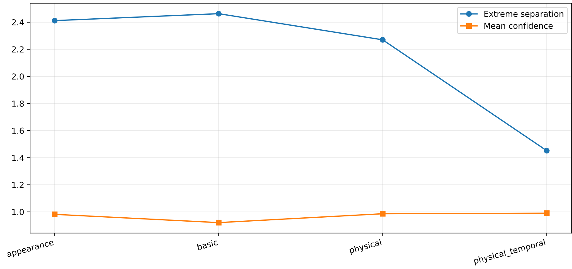
Feature ablation for anchored GMM
