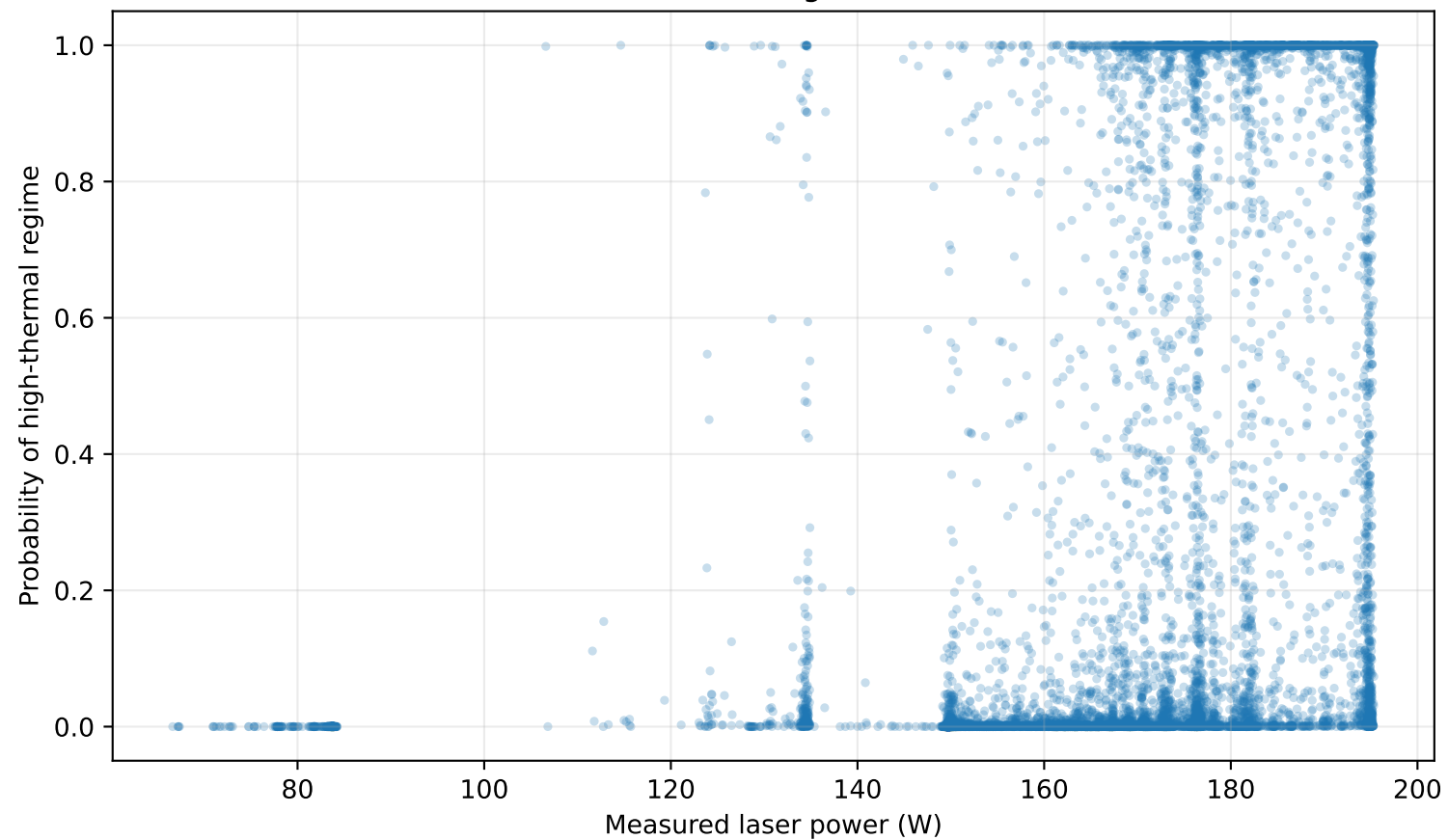
Probabilistic regime score
