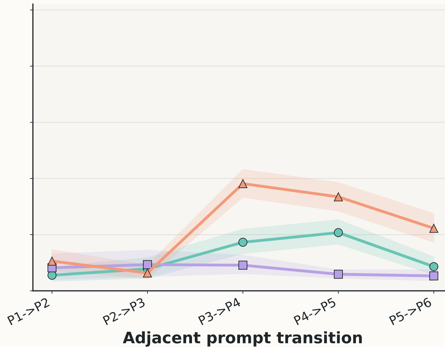
EBM-NLP
