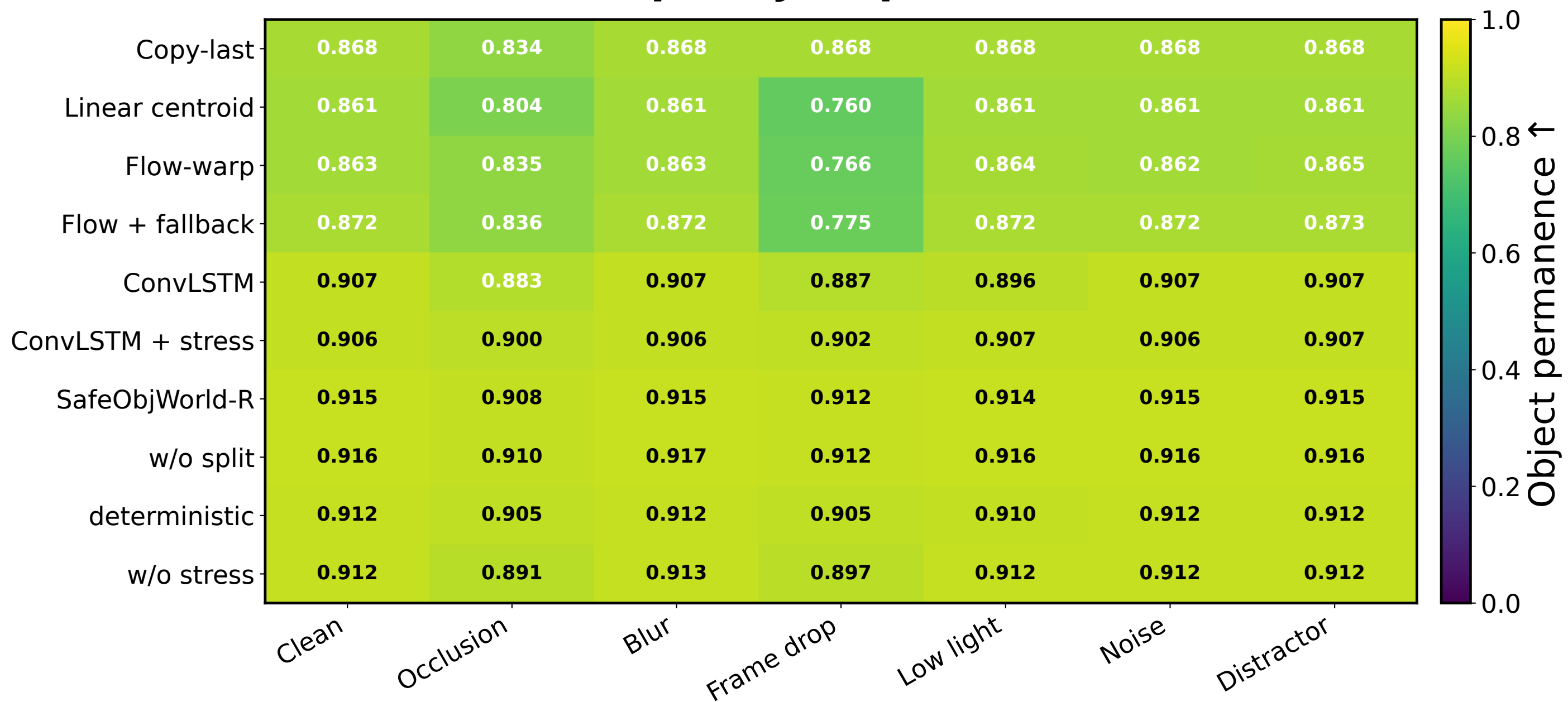
Stress Heatmap: Object permanence ↑, H=10
