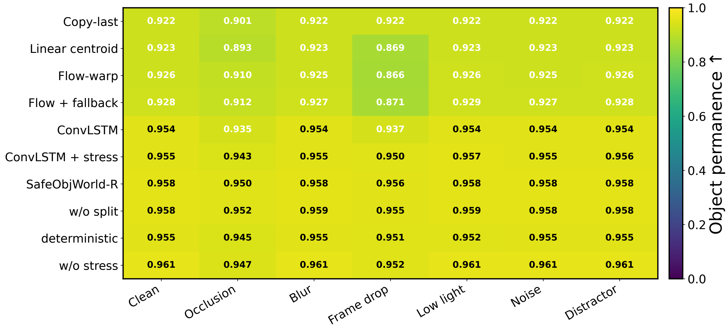
Stress Heatmap: Object permanence ↑, H=5
