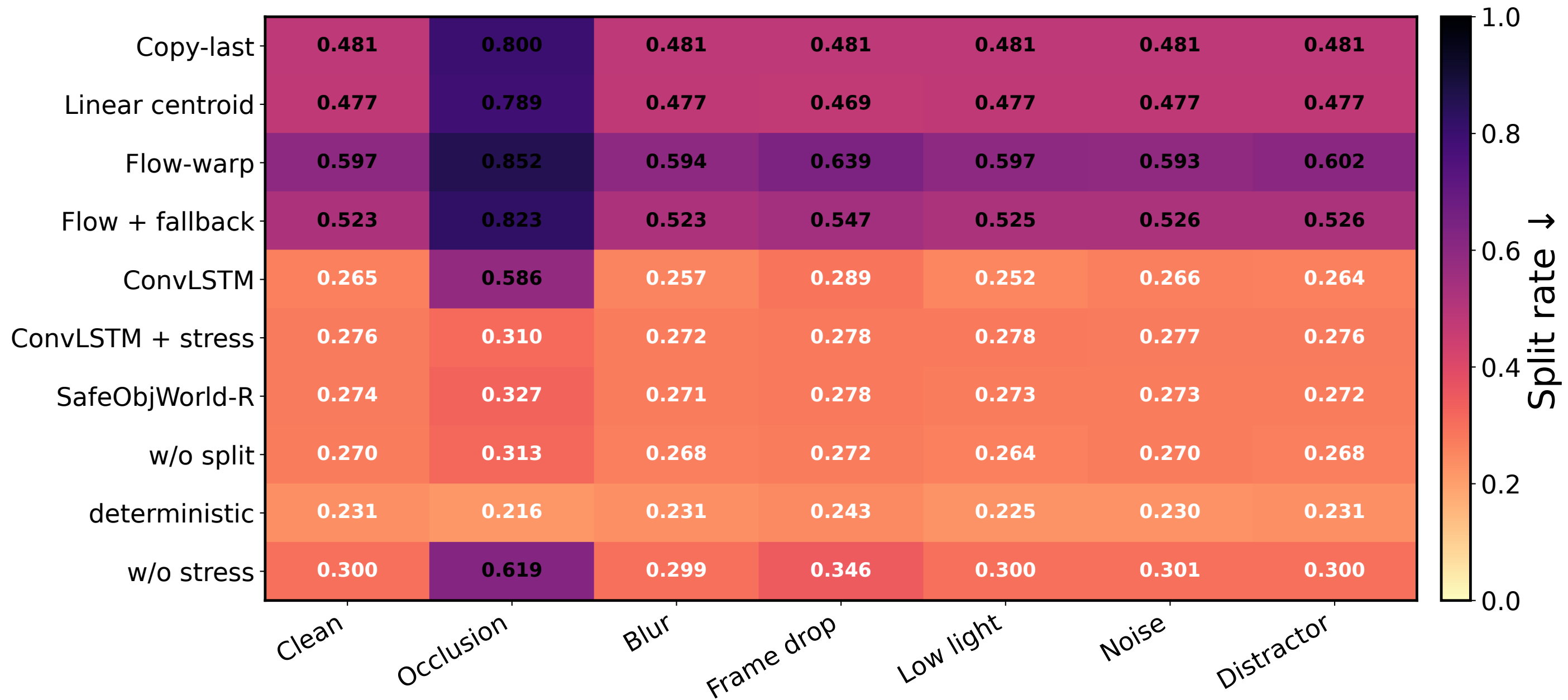
Stress Heatmap: Split rate ↓, H=10
