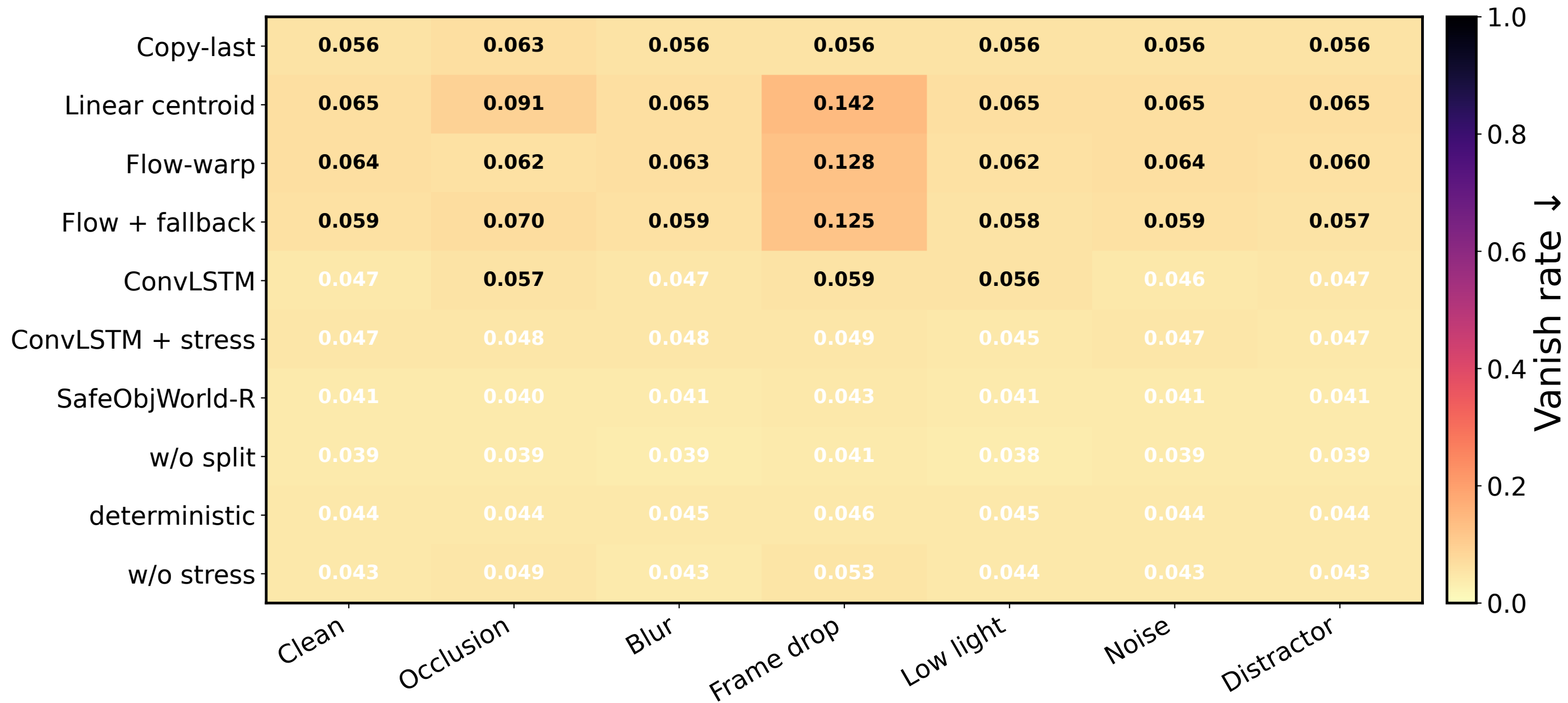
Stress Heatmap: Vanish rate ↓, H=10
