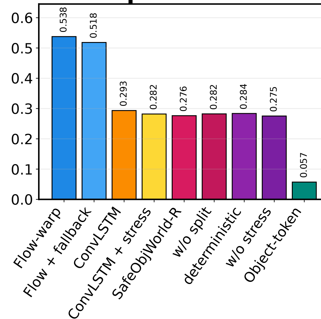
Split rate ↓
