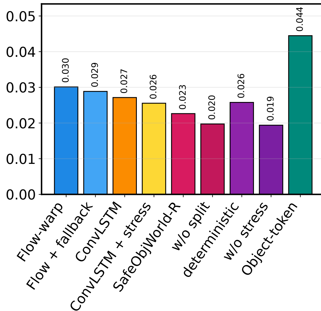
Vanish rate ↓
