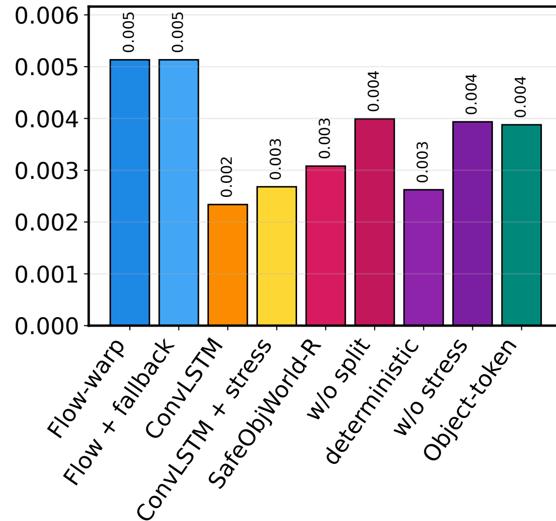
Hallucination ↓
