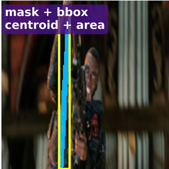
Object-centric state
