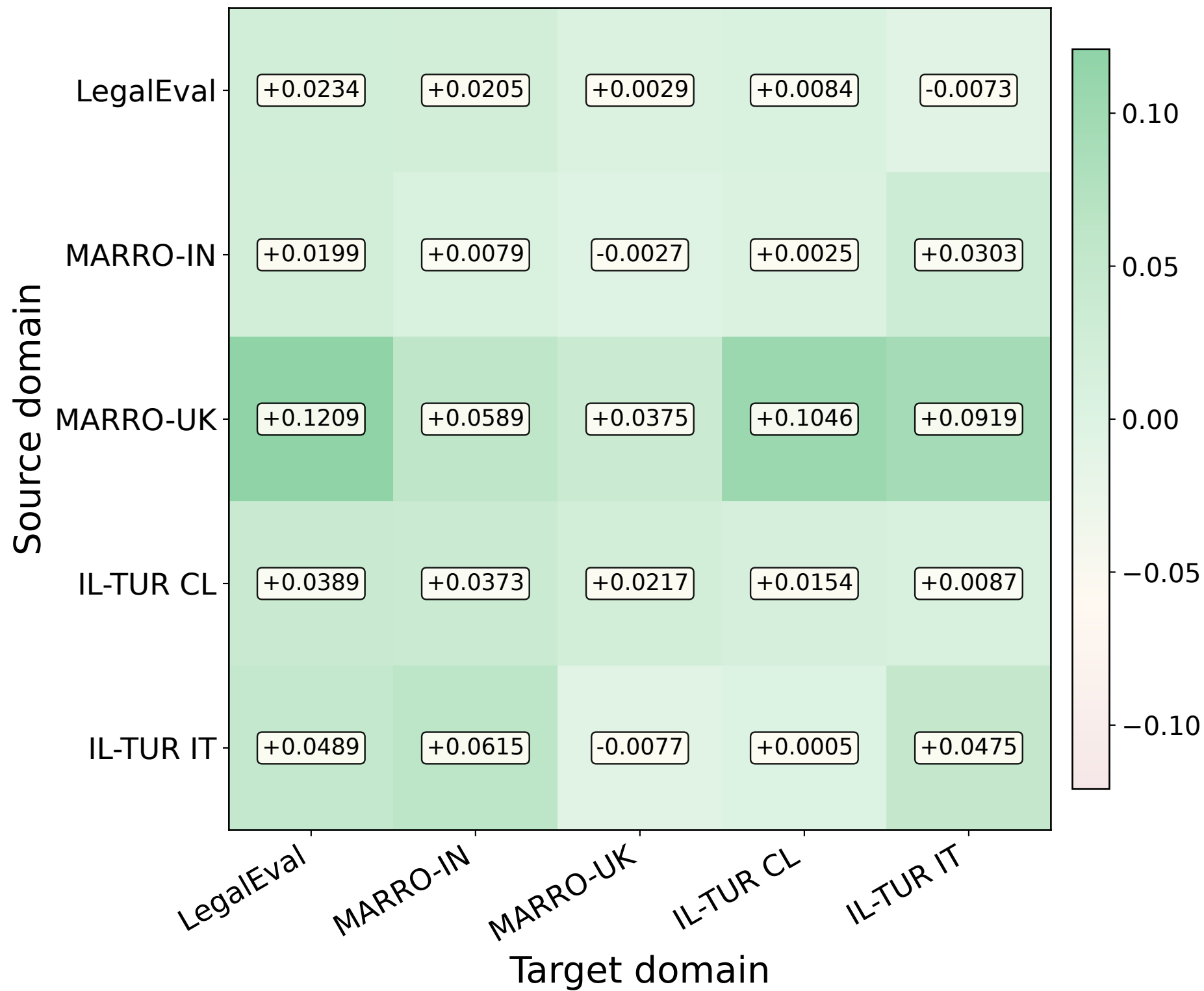
Role Adapter minus Shared LoRA
