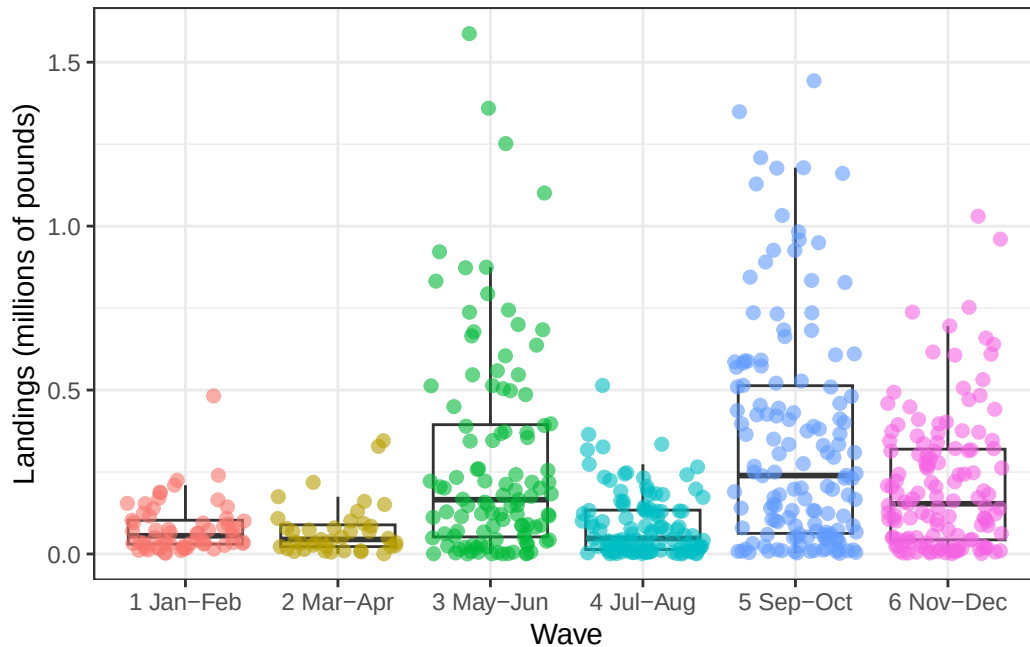
Figure 12.3: White Shrimp Landings in GA and SC, by wave. These landings are reported as head-off weights (pounds) by state. They were not added or averaged here; each point represents a number for a state in a given year.
