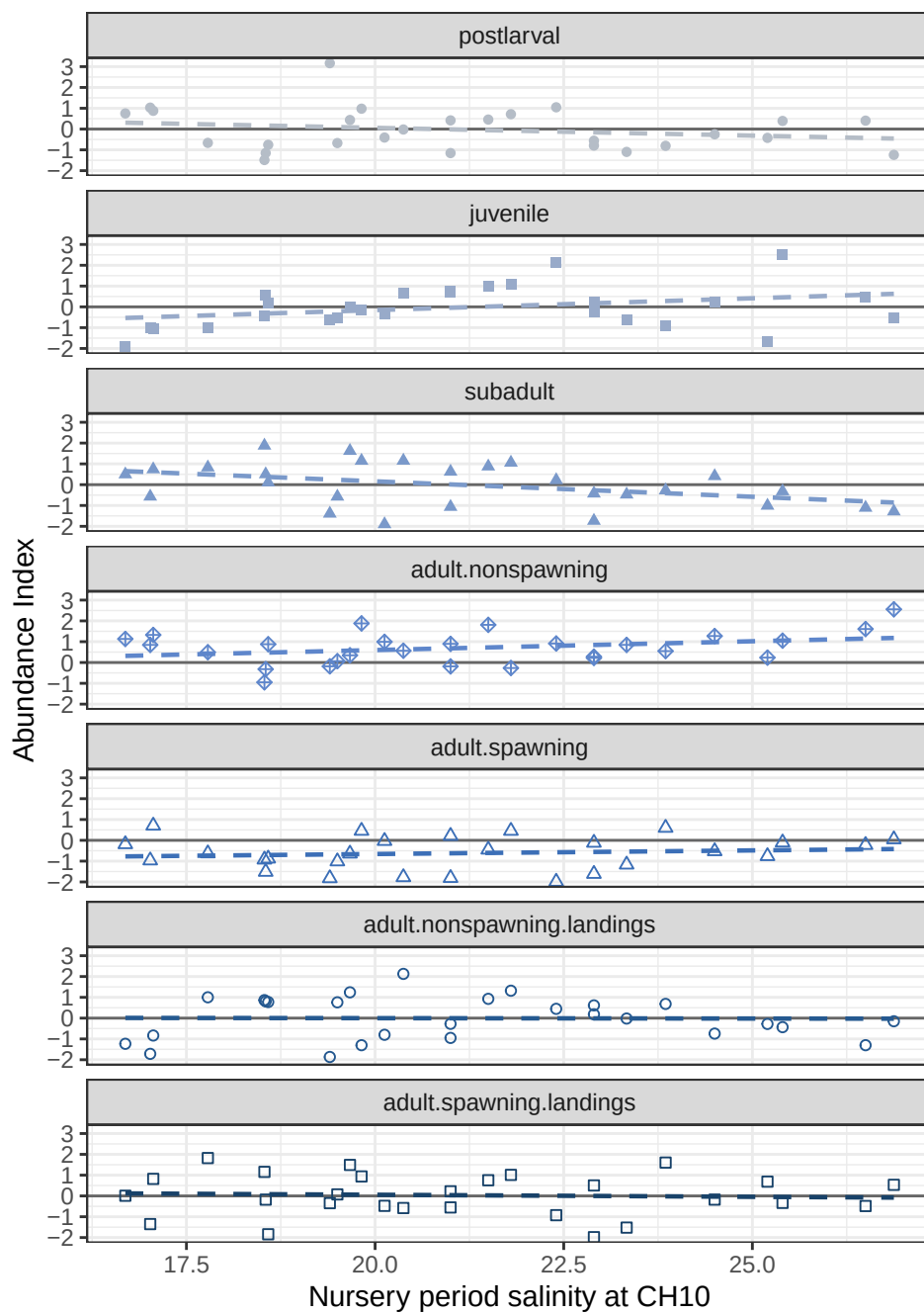
Figure 17.6: Graphic of white shrimp abundance index at each life stage vs. nursery period salinity at CH10. Dashed lines show a linear smooth, whether correlations were significant or not.
