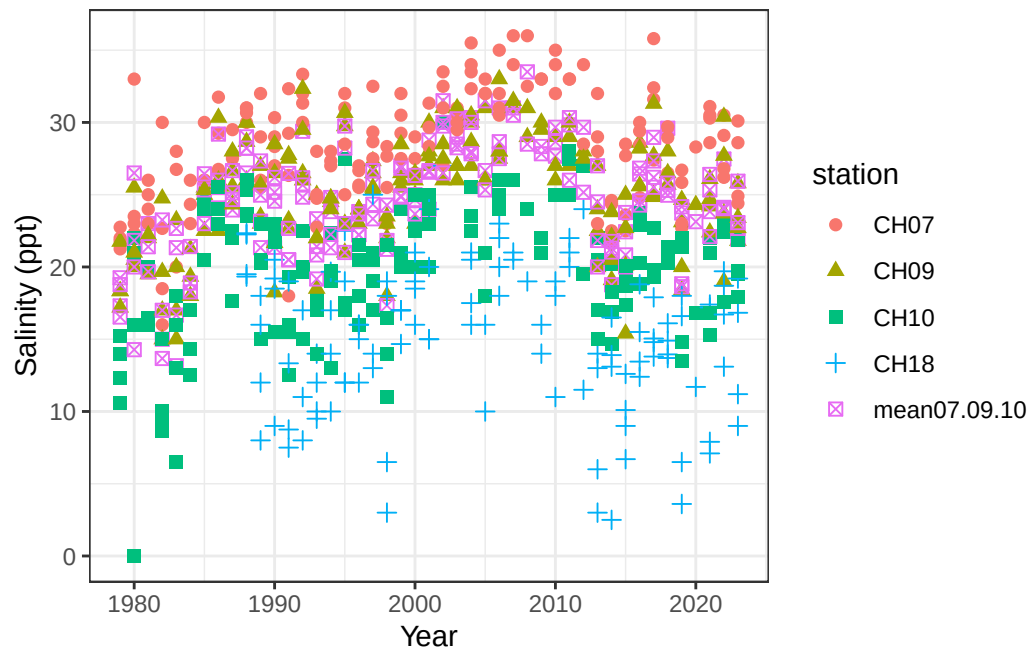
Figure 14.1: All brown shrimp nursery period salinity values by shrimp year
