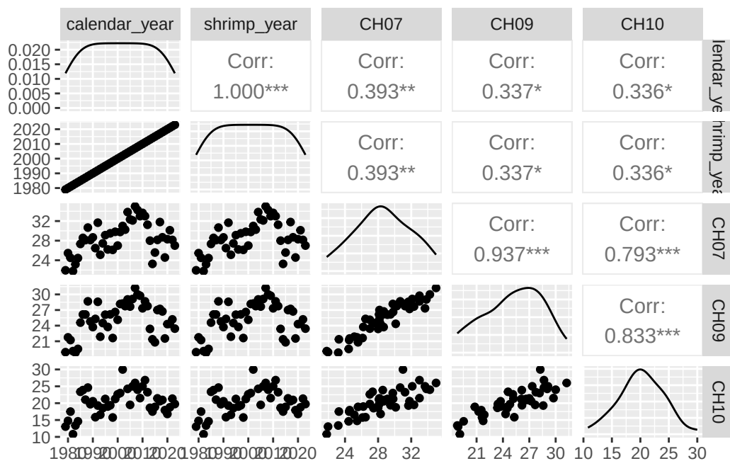
Figure 14.3: Pairs plot of brown shrimp nursery period salinities (mean for each year) at the different stations
