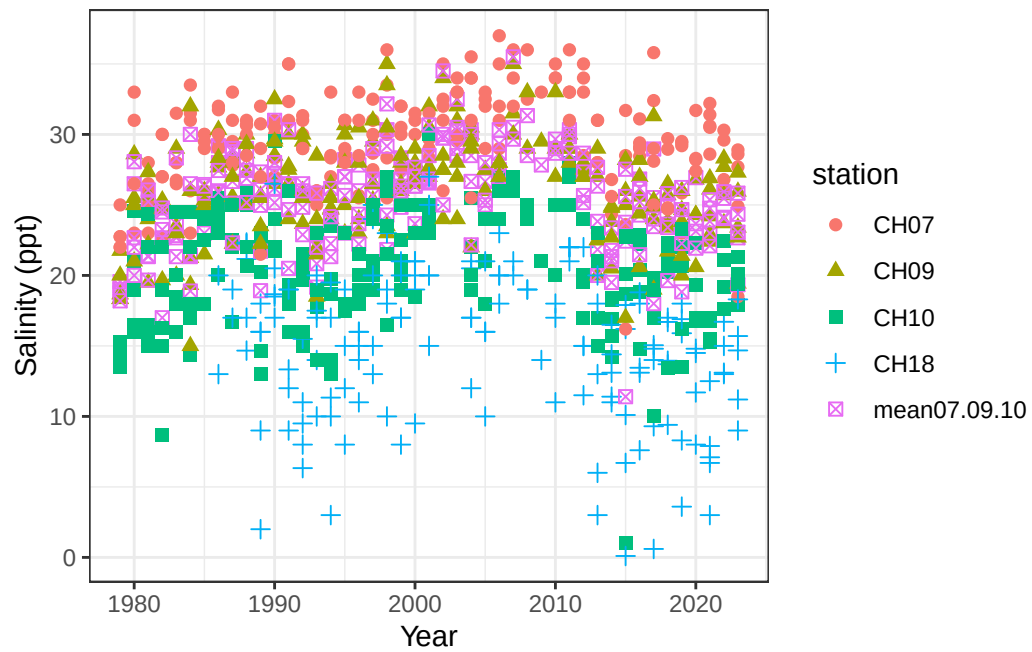
Figure 14.4: All white shrimp nursery period salinity values by shrimp year
