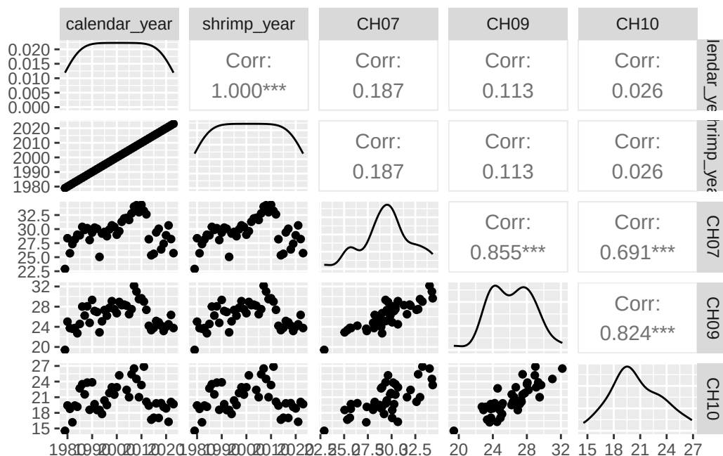
Figure 14.6: Pairs plot of white shrimp nursery period salinities (mean for each year) at the different stations
