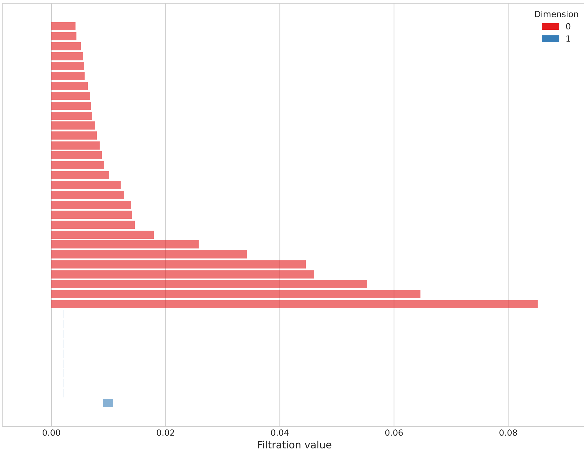
Barcode of US Indices - Window 5303
