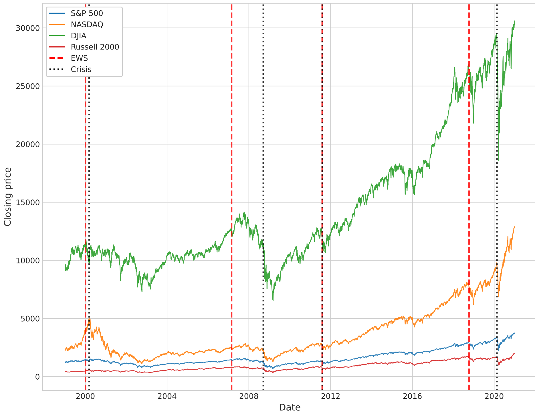
US Indices with detected EWS and crises
