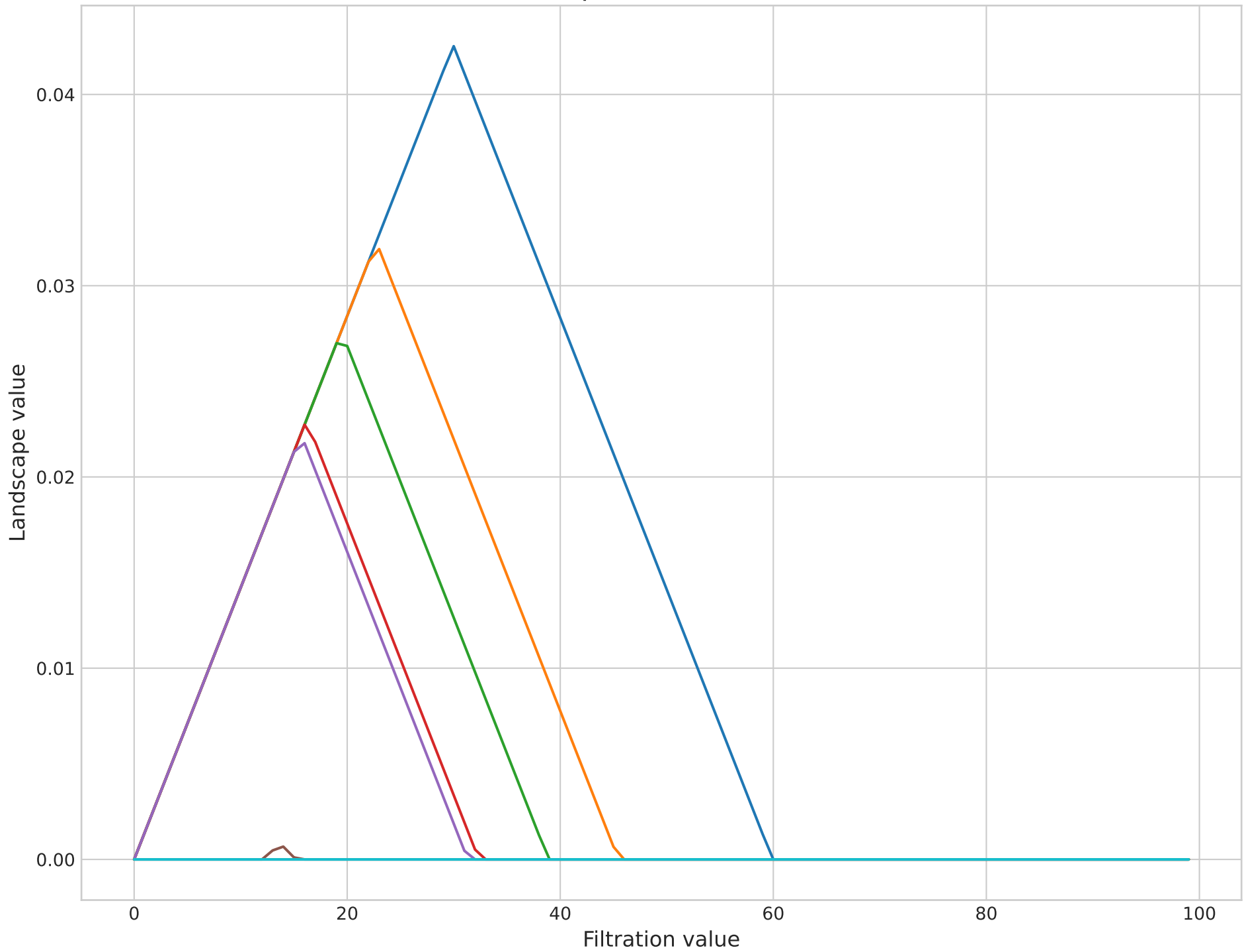
Persistence Landscape of US Indices - Window 5303
