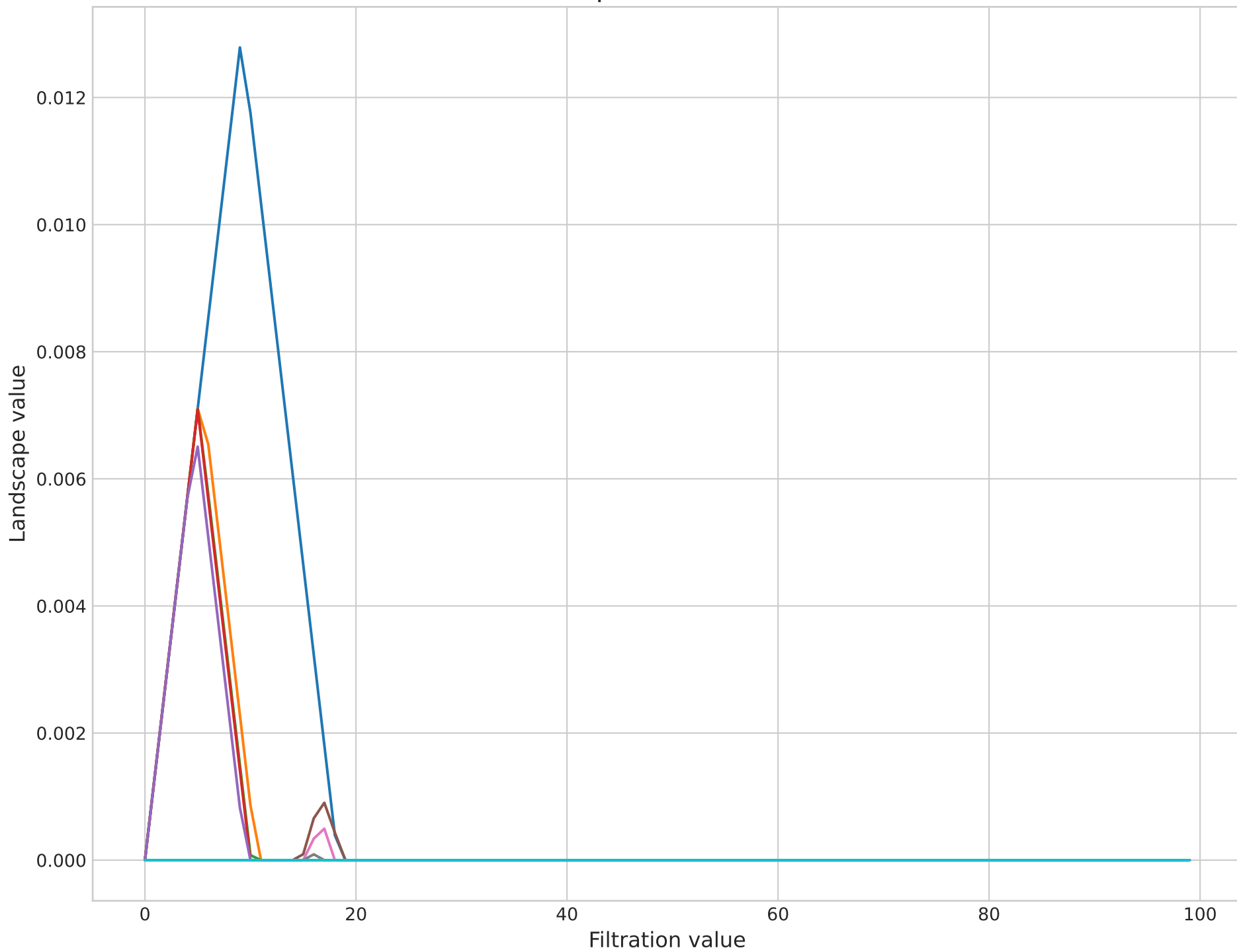
Persistence Landscape of US Indices - Window 585
