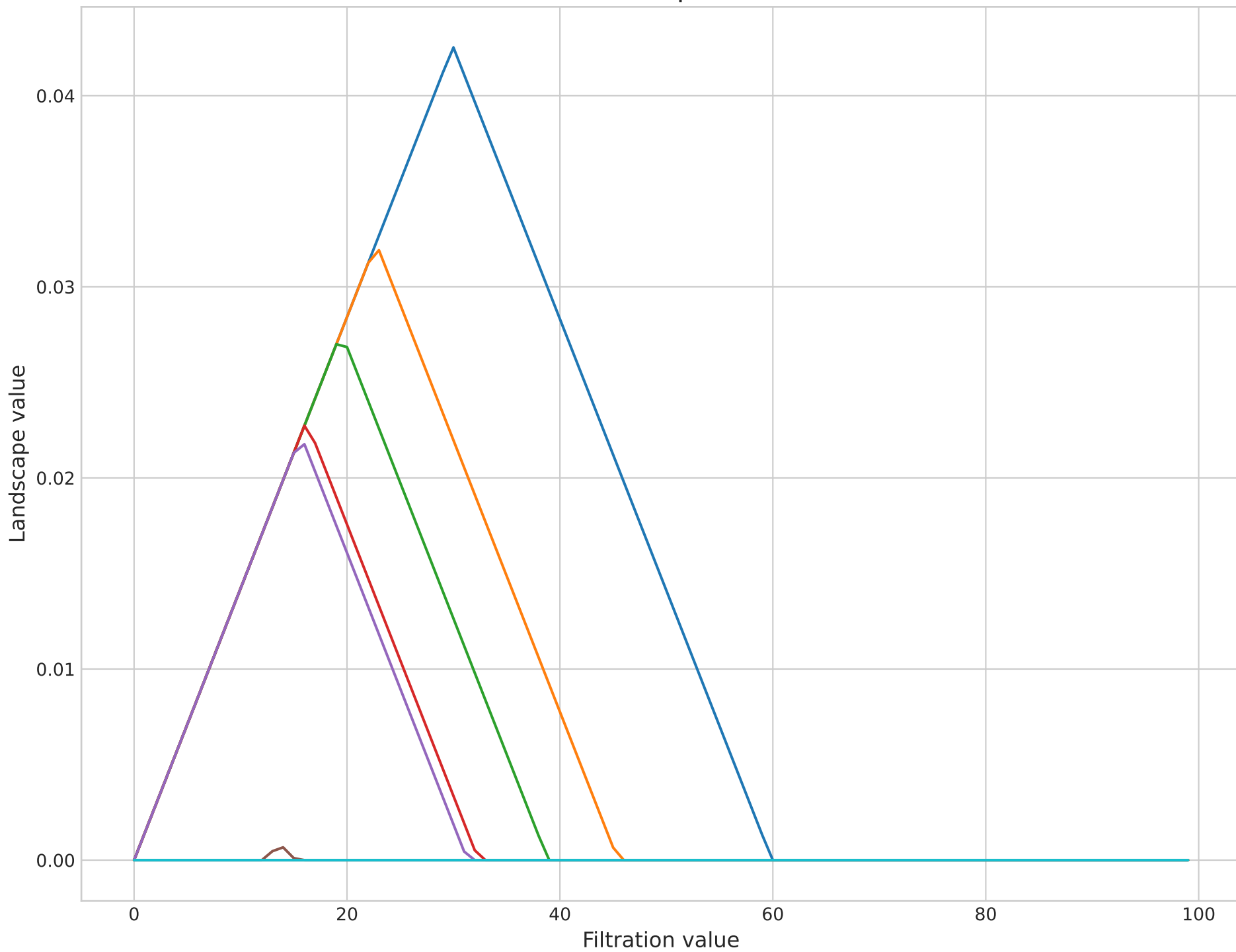
Persistence Landscape - Window 5303
